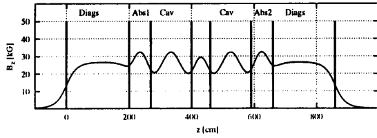
Figure 2: Longitudinal magnetic field on axis.
