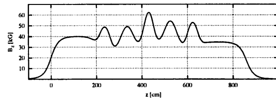
Figure 6: Alternative longitudinal magnetic field.
