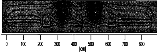
Figure 1: Solenoid layout and magnetic field lines computed with POISSON. The system has a cylindrical symmetry with respect to the horizontal axis.
