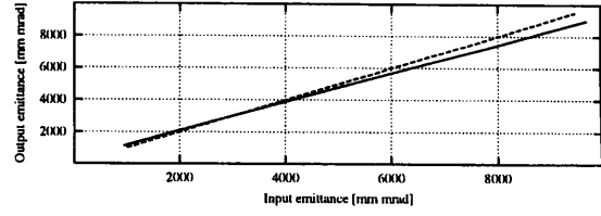
Figure 4: Output emittance vs input emittance (r.m.s., normalized) at 200 MeV.
