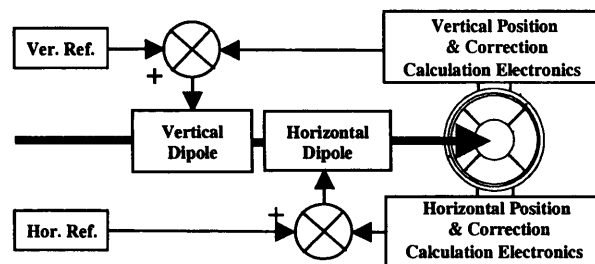
Figure 2: Block schematic of the feedback system.
