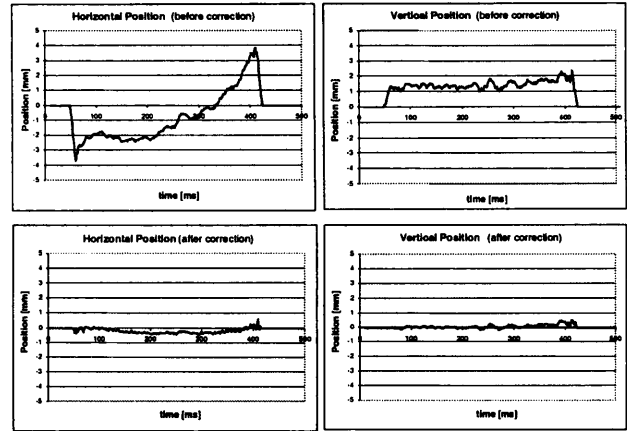
Figure 6: Beam position as function of time before and after correction.
