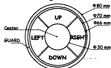
Figure 1: Layout of the 'Centroid' detector.
