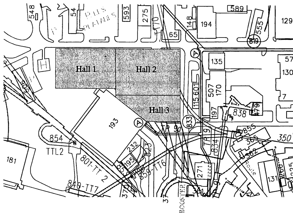
Figure 1: A conceptual plan of where the future CERN second-generation RNB facility could be located. Hall 1 would hold the storage ring complex and Hall 2, the post-accelerator and the multi-segmented detectors. In Hall 3 a class A laboratory for handling of radioactive targets would be housed. The three target stations would be accessed directly from Hall 3 avoiding any unnecessary transport of radioactive material on the site.
