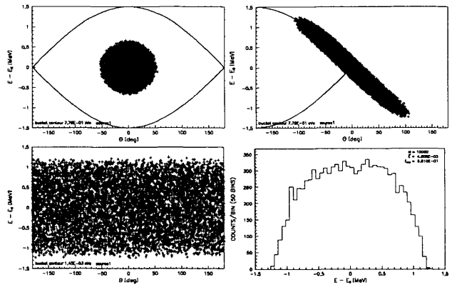
Figure 3: ESME simulation of the RF phase jump with 250 MeV protons and debunching before extraction.
