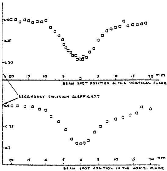
Fig. 1. Scan of BNL aluminum foil SEC.
