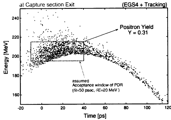
Figure 3: Longitudinal phase space at 204 MeV.
