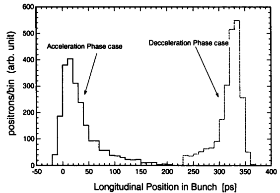
Figure 5: Bunch distribution for both phases.
