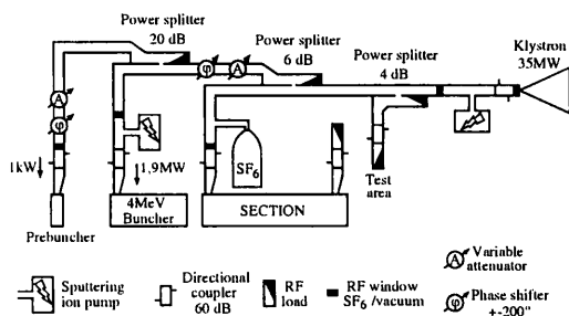
Figure 4: Power RF network
