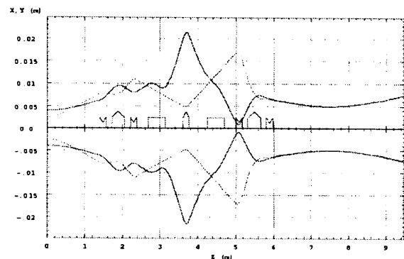
Figure 5: Beam transport calculations
