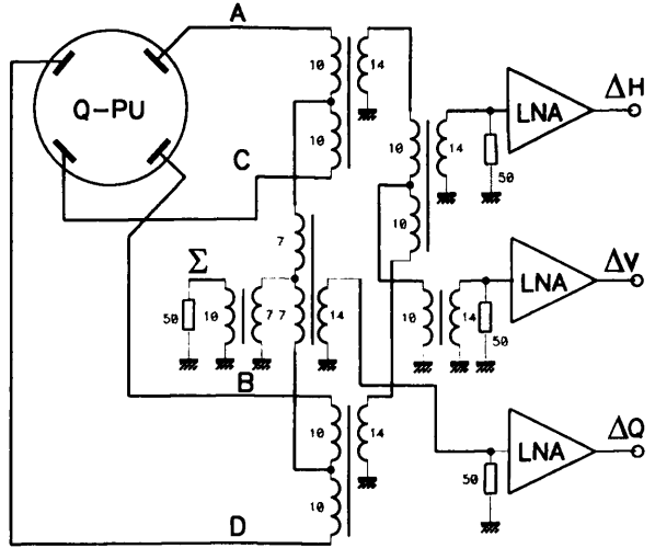
Figure 3: Analog signal chain.
