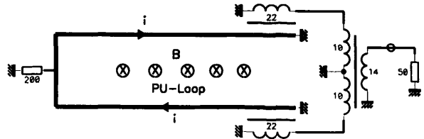
Figure 2: Schematic layout of one antenna loop
