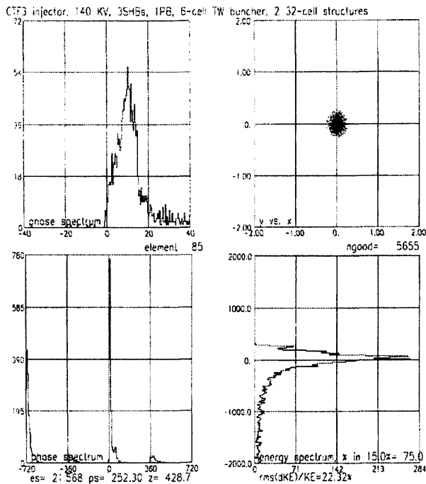
Figure 3: PARMELA results.
