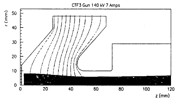
Figure 2: EGUN results for the CTF3 gun.
