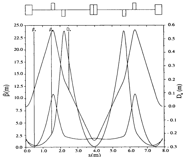
Figure 1: Optical functions for R_{56} = -0.04 m.
