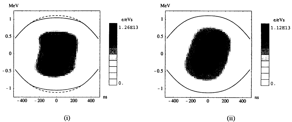
Figure 2: Phase space reconstructions (i) with and (ii) without space charge. Note the different density scales.
