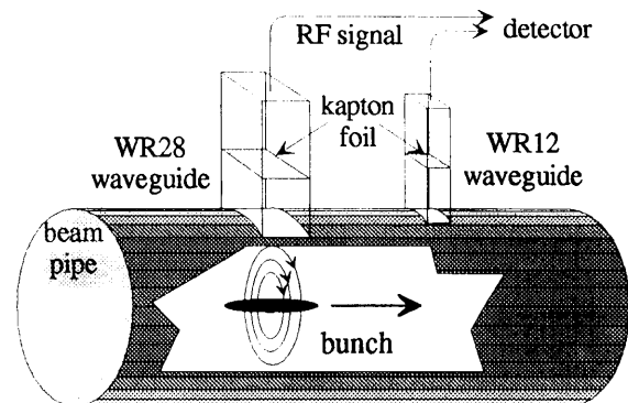
Figure 1: Layout of the coupling between the beam pipe and the waveguide.
