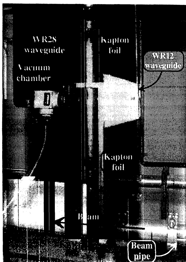
Figure 2: Beam pipe-waveguide coupling as installed in the CTF drive linac.
