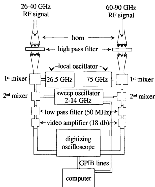
Figure 3: Detection system.
