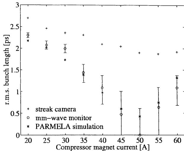
Figure 5: Bunch length measurements.
