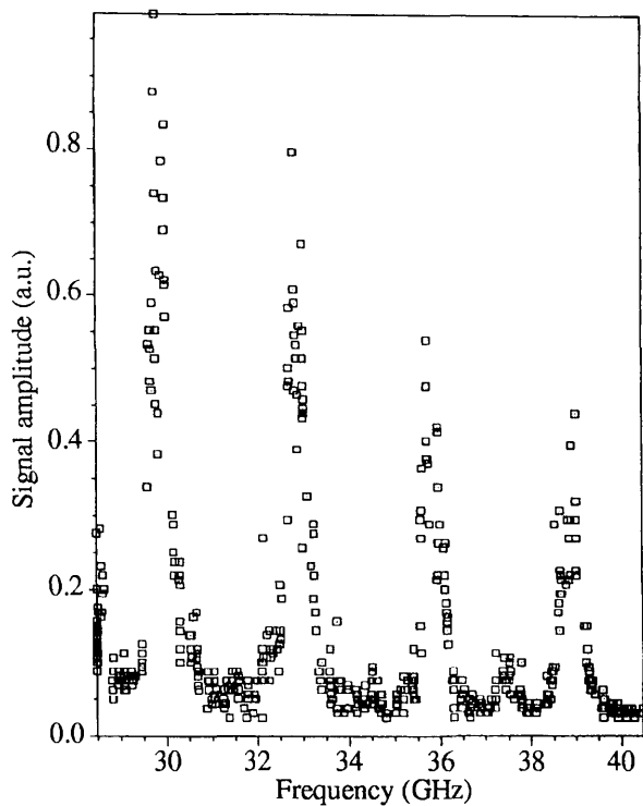
Figure 4: Measured frequency spectrum for a train of 8 bunches.
