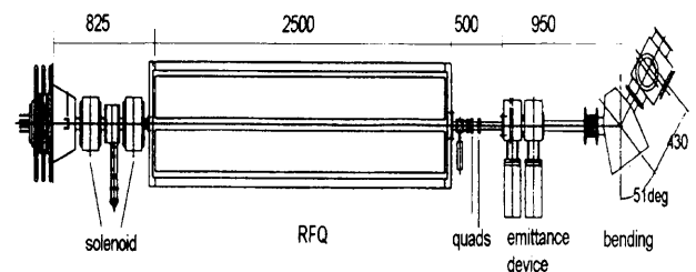
Fig. 3 The experimental set-up consisting of a proton source, two solenoids, the RFQ, and a measurement line. Dimensions are in mm.
