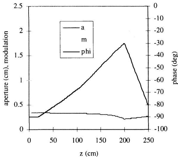
Fig. 1. Variation of RFQ aperture, modulation and phase vs. length. Phase and modulation are tapered down in the last section in order to limit the output energy to 100 keV/u for the first phase of the experiment.
