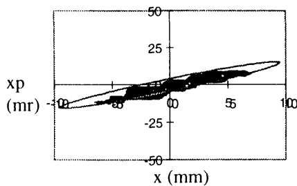
Fig. 4 Measured horizontal emittance , the solid line represents the calculated ellipse.
