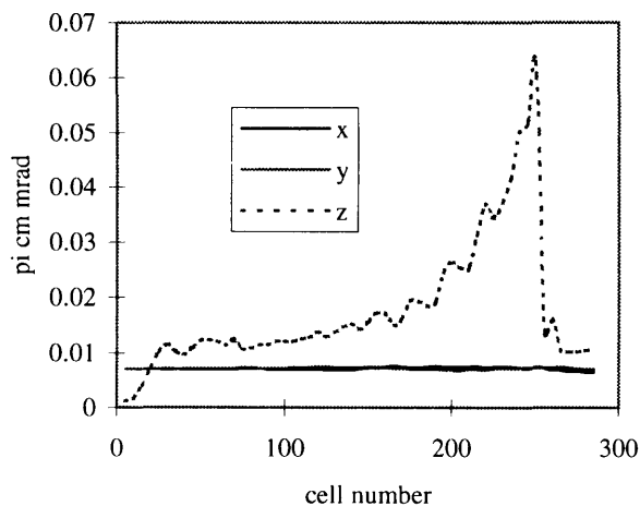
Fig. 2 Transverse and longitudinal emittance evolution for a mono-species beam.
