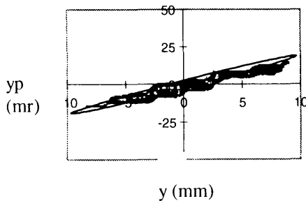
Fig. 5 Measured vertical emittance , the solid line represents the calculated ellipse.
