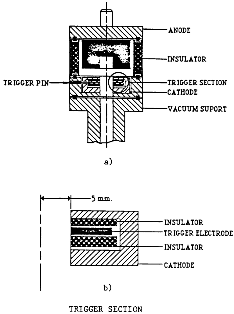
Fig. 4 - Schema of the slide-spark triggered pseudo-spark switch (a), and enlargement of the trigger section (b). The discharge is ignited by applying a high voltage pulse (of typically 2 kV) to the trigger electrode, causing the surface of the thinner insulator to flash over.
