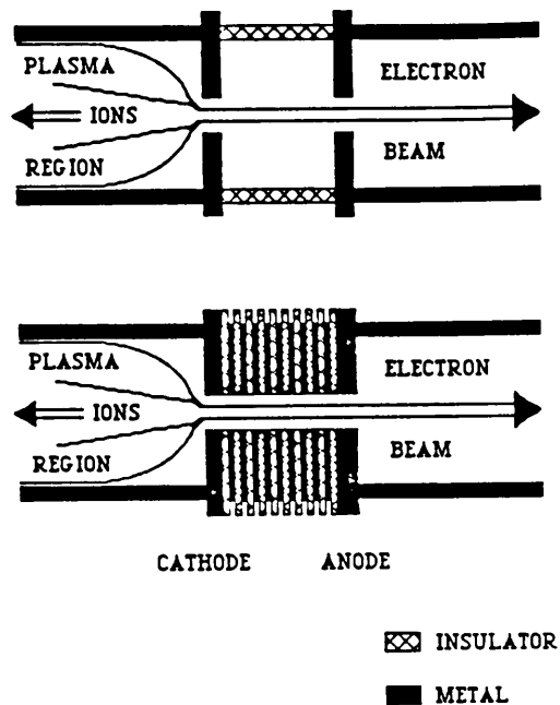
Fig. 1 - Schematic of single-gap (top) and multigap (bottom) pseudo-spark chambers, showing the discharge geometry.
