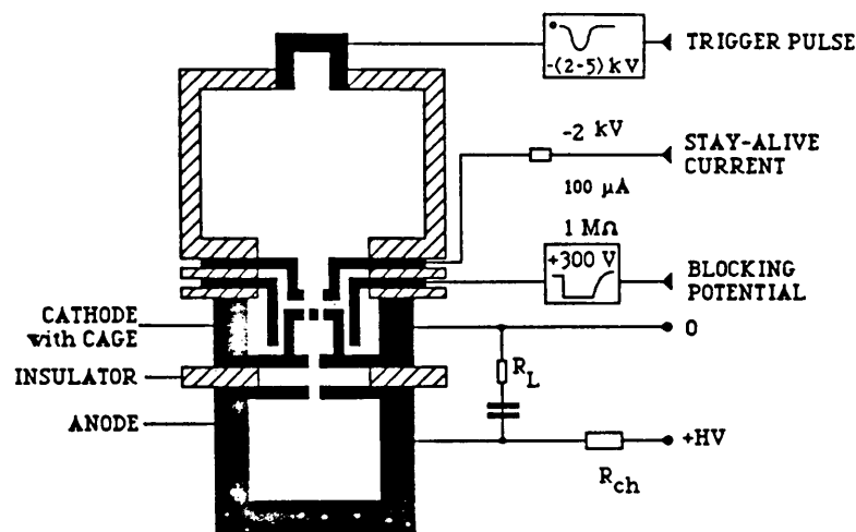
Fig. 2 - Experimental pseudo-spark switch design for pulsed glow discharge triggering, and electrical circuit. To trigger the switch, the blocking potential of several 100 V is driven to zero, and a negative high voltage pulse of 2 to 5 kV in amplitude and several microseconds duration is simultaneously applied to the trigger electrode.
