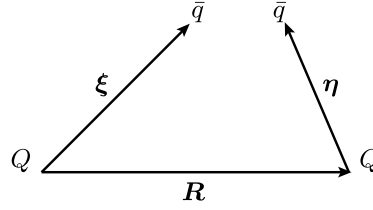
Fig. 1. The heavy quarks are separated by the vector \mathbf{R} . The vectors \xi and \eta have their application points at the two heavy quarks.
