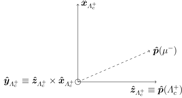
Figure 5: Definition of the \Lambda_c^+ polarization system. The \hat{\mathbf{y}}_{\Lambda_c^+} axis is orthogonal to the page, towards the reader.
