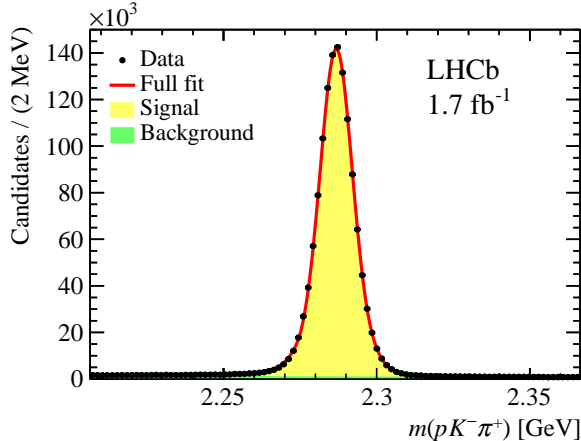
Figure 1: Invariant mass distribution of selected pK^-\pi^+ candidates from the total dataset. The results from the fit described in the text are also shown.
