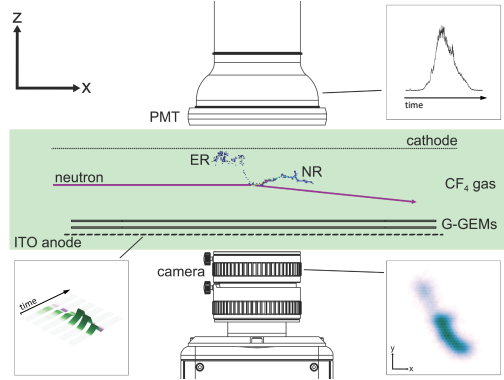
Figure 1: Schematic representation of the MIGDAL experiment showing the OTPC exposed to neutrons, with interactions in the low-pressure \text{CF}_4 gas amplified by a double glass-GEM system; the active volume of the OTPC is approximately 10 \times 10 \text{ cm}^2 by 3 cm in the drift direction; neutron interactions take place in a volume \approx 9 \times 9 \text{ cm}^2 by 1.3 cm. Optical signals are recorded by an external camera and a photomultiplier tube, while amplified track ionisation is detected by an ITO-strip anode. An example 2D-projected Migdal event (scaled 10 \times ) is shown, featuring a 5-keV electron and a 150-keV fluorine nuclear recoil originating from the same vertex – simulated using Degrad [48] and SRIM [49] plus Garfield++ [50], respectively. Illustrative signals in the various detector systems are also shown.
