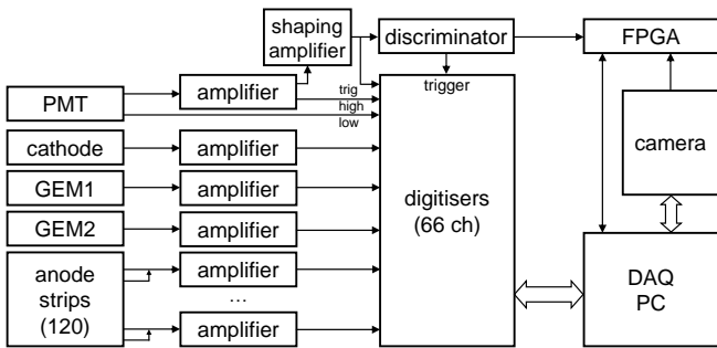
Figure 11: Box diagram highlighting the three main data acquisition elements: digitisers, camera and FPGA – controlled and read out by a common PC.
