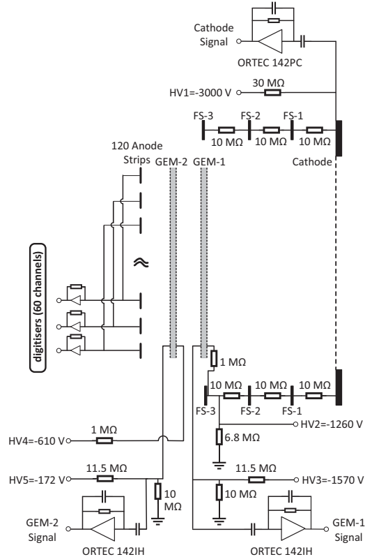
Figure 9: Electrical circuit showing the OTPC bias and readout.
