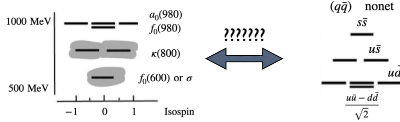
FIG. 11. Mass spectra of the scalar multiplets vs. a typical (q\bar{q}) nonet.
