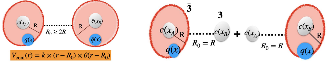
FIG. 24. (left) Confined orbitals. (right) Ground state of the doubly charmed baryon.
