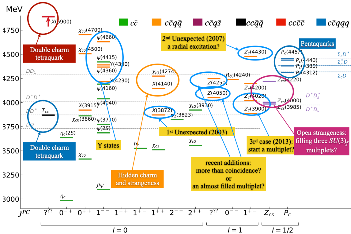
FIG. 1. Anticipated and unexpected charmonia. In green the observed ordinary charmonium lines. Compilation and figure adapted from [2].
