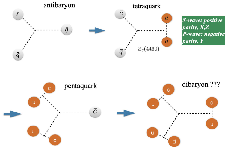
FIG. 3. Color strings in multiquark states.
