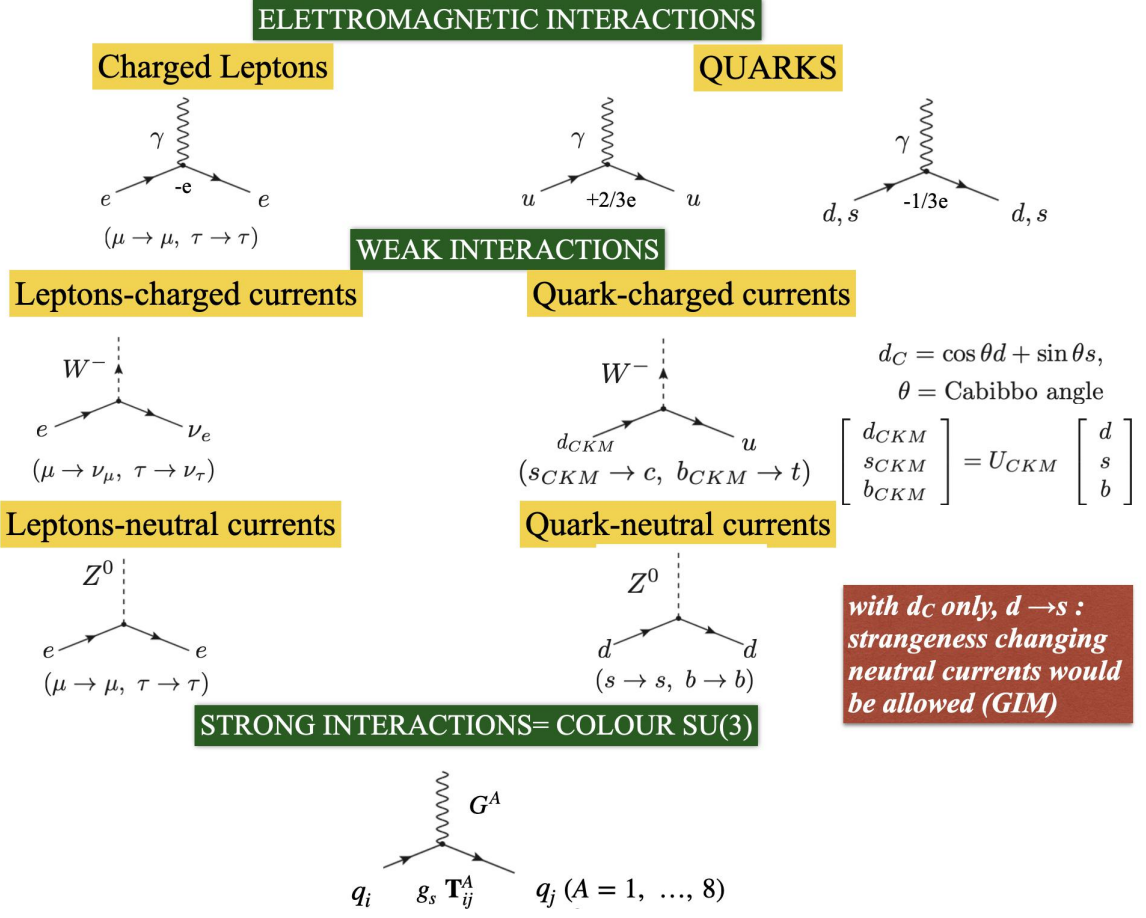
FIG. 8. Elementary interactions of quarks with the gauge fields of the Standard Theory, with gauge group SU(2)_L \otimes U(1)_Y \otimes SU(3)_c .
