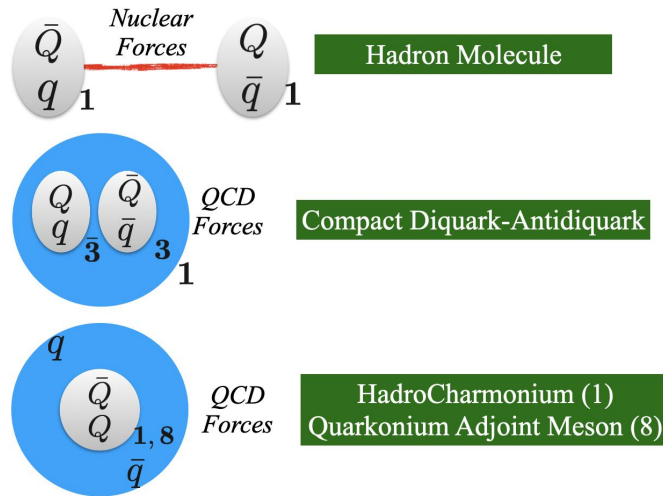
FIG. 4. Schematic representation of hadron molecules (see [10]), compact tetraquarks (see [11]), hadrocharmonium and quarkonium adjoint mesons (see [8, 9]).
