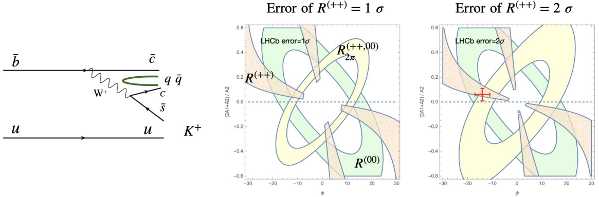
FIG. 23. Left: diagram for B -decay to a six-quark state. Right: contour plots of the ratios in (80)-(82).
