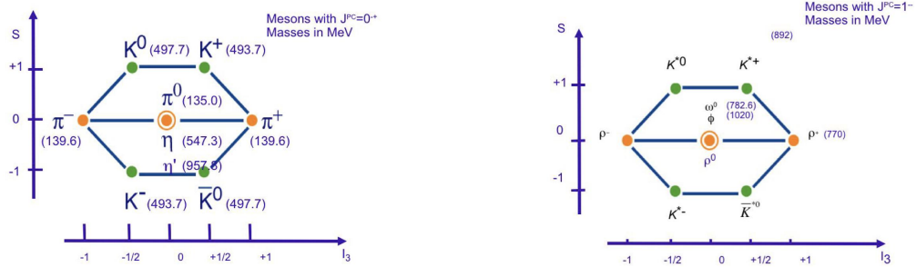
FIG. 5. The Eightfold Way: (left) the octet of pseudoscalar mesons; (right) the octet of vector mesons.
