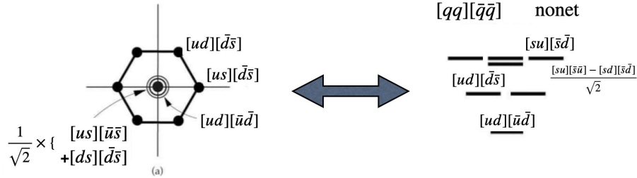
FIG. 12. Mass spectrum of Jaffe's tetraquark.
