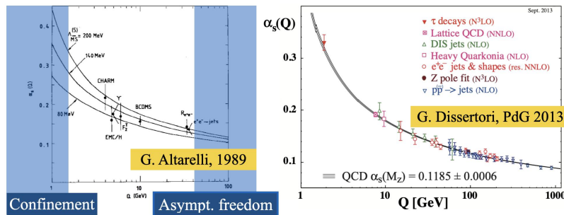
FIG. 7. Asymptotic Freedom is signalled by the decrease of the coupling constant at large q^2 .
