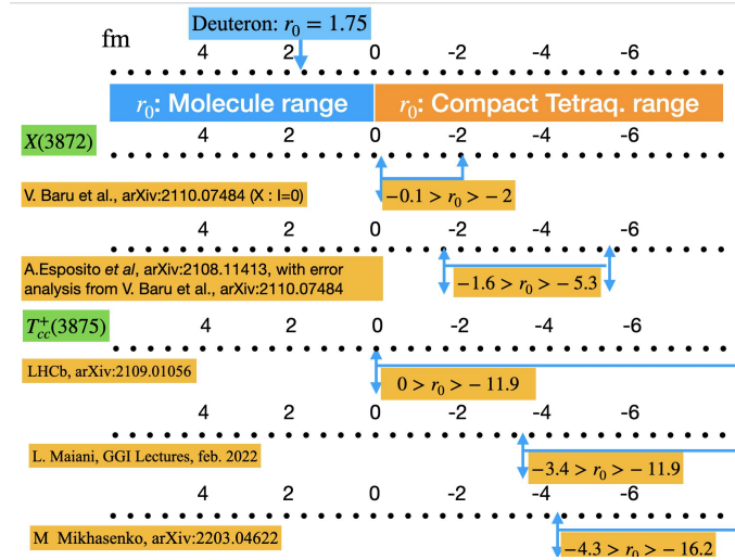
FIG. 45. Compilation of recent reterminations of the effective radius, r_0 , compared to the effective radius of the Deuteron.
