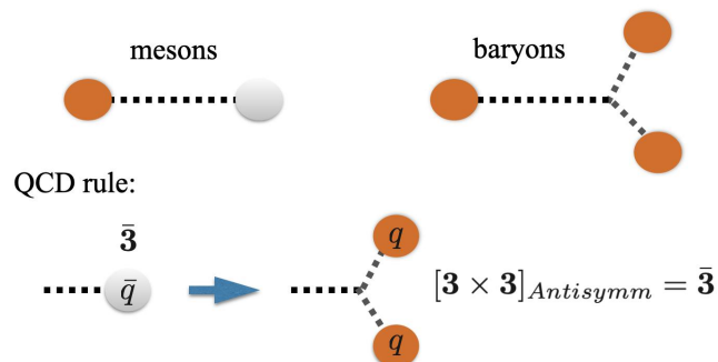
FIG. 2. Color strings in ordinary mesons and baryons.
