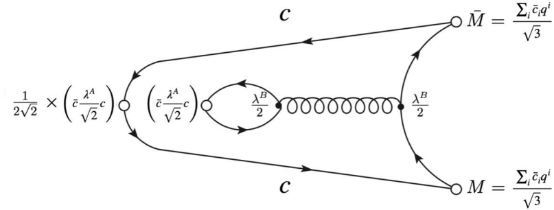
FIG. 21. Annihilation of color octet, spin 1 quark pairs.
