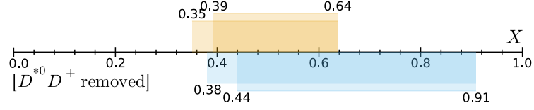
FIG. 44. \mathcal{T}(3875) : intervals for the compositeness parameter X of at 90(95) % confidence level. M. Mikhasenko, ArXiv:2203.04622.
