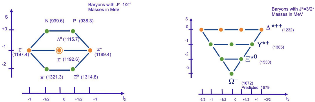
FIG. 6. The Eight Fold Way:(left) the octet of spin-1/2 baryons; (right) the decuplet of spin-3/2 baryons.
