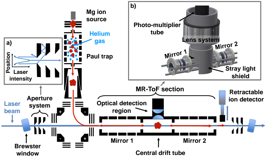
Fig. 1. Simplified schematics of the MIRACLS proof-of-principle experiment with close-up insets of the laser-entrance aperture system (a) and the stray light shield of the optical detection region (b). For details, see the text.
