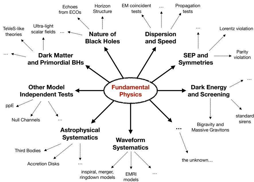
Figure 1 Schematic diagrams of topics of relevance to the Fundamental Physics WG of the LISA Consortium. Some of these topics overlap naturally with other WGs, such as the Waveform modelling WG, the Astrophysics WG and the Cosmology WG.
