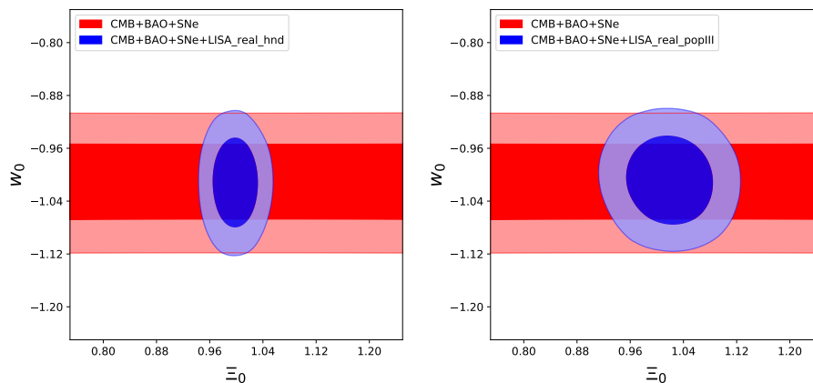
Figure 3 The 1\sigma and 2\sigma contours of the two-dimensional likelihood in the (\Xi_0, w_0) plane, with the combined contribution from CMB+BAO+SNe (red) and the combined contours from CMB+BAO+SNe+LISA standard sirens (blue). Left: heavy seeds and no-delay (“hnd”) scenario; right: “pop III” seeds. From Belgacem et al. (2019c).
