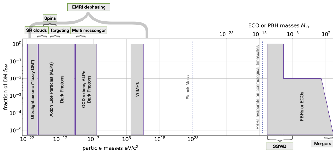
Figure 2 Overview of key DM candidates (Bertone and Tait, 2018; Bertone et al., 2019; Giudice, 2017). Currently excluded ranges of particle masses and DM fractions f_{DM} are indicated in white. Parameter regions where LISA observations may provide constraints are gray coloured. We see that the masses of DM particle candidates remain currently very much unconstrained and that DM particles of any allowed mass can make up any fraction ( f_{DM} \leq 1 ) of the DM. Macroscopic DM candidates such as PBHs and ECOs are constrained by current observations but may still constitute 100% of the DM in the range 10^{-16} - 10^{-11} M_{\odot} . Approximate regions where LISA can contribute to constraints are bracketed above and below the plot with a brief description - see the text for more details.
