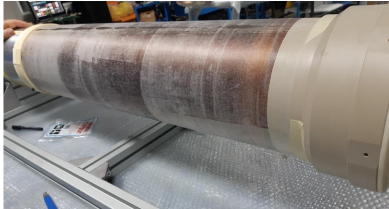
Figure 3.17: Fiberglass deposition on cathode.
