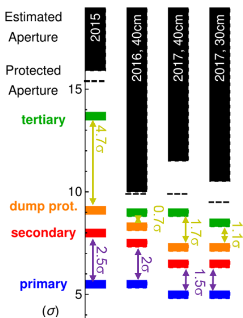
Figure 1: Evolution of the betatron collimator settings over past years during Run II.
