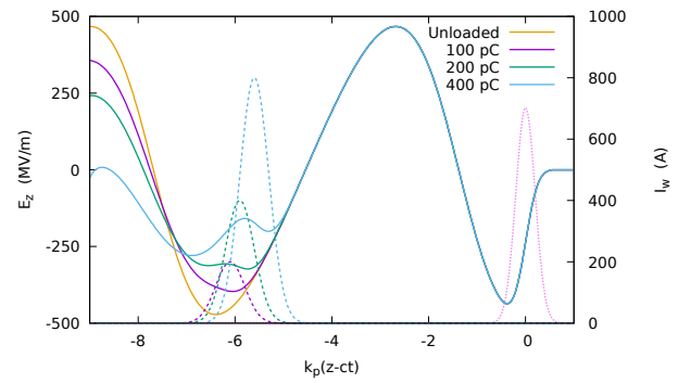
Figure 4: Accelerating field E_z (solid lines) and witness current (dashed lines) taken at the start of the simulation for witness charges of 100, 200 and 400 pC, as well as for the unloaded wakefield. The drive bunch is centred at z-ct = 0 and is illustrated by the violet dotted line (not to scale, peak current 17.5 kA). For each witness charge, the position is chosen to minimize the relative RMS energy spread after 10 m.
