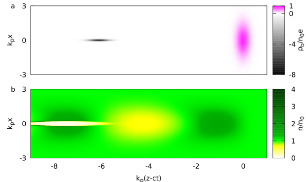
Figure 1: The toy model consists of a) a short, positively charged driver (violet), trailed by the witness electron bunch (black). The two are coupled by b) the plasma response, with the driver exciting a quasilinear wake. If the witness is sufficiently dense, it will drive a blowout.
