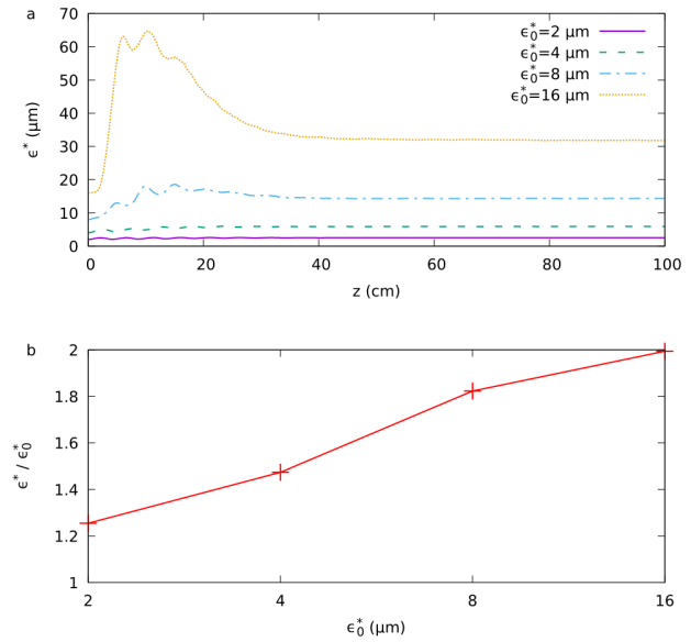
Figure 2: Influence of initial emittance on emittance growth. a) Witness emittance over the first metre of acceleration for different initial emittances. b) Witness emittance after 10 m acceleration, relative to the initial emittance.
