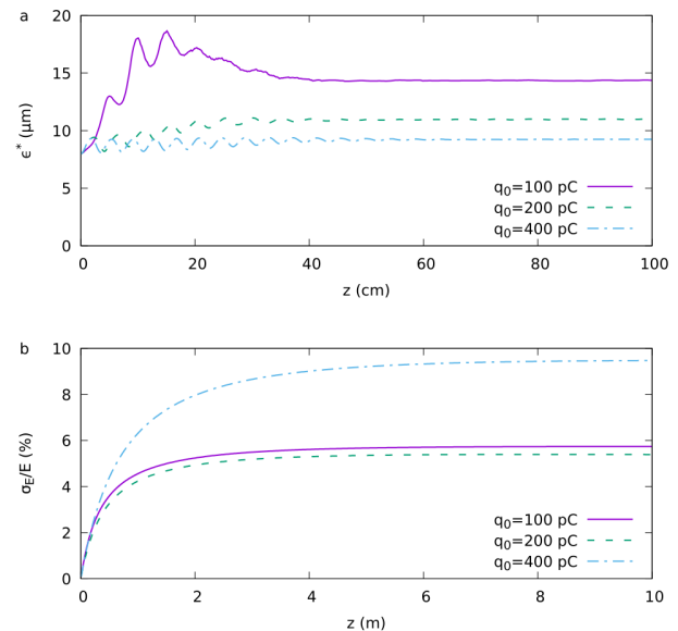
Figure 5: Influence of initial charge on acceleration quality for an initial emittance of 8 \mu\text{m} . a) Witness emittance over the first metre of acceleration for different initial charge, and b) Relative witness energy spread over the full 10 m acceleration.
