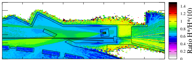
Figure 3: 160 MeV H^- on the LBE beam dump (tilted rectangular object), generating prompt radiation in the area and penetrating into the PS Booster area (left side). The heat map is showing the ratio H^* to H^*(10) .
