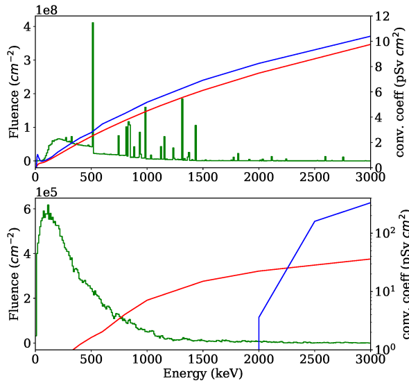
Figure 2: Photon (top) and electron (bottom) decay radiation fluence spectra of the irradiated steel target, scored 1 hour after the end of the irradiation (left abscissa). The conversion coefficients for H^* (red) and H^*(10) (blue) are overlaid (right abscissa).
