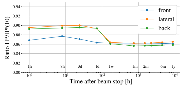
Figure 4: Dose rate ratios H^* to H^*(10) from decay radiation at different locations in front, laterally and at the back of the LBE dump against decay times between 1 hour and 1 year.
