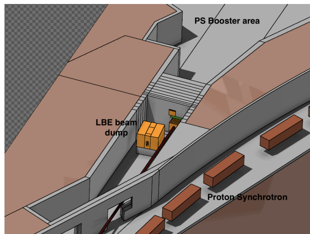
Figure 1: The LBE beam dump and PS Booster shielding and area.
