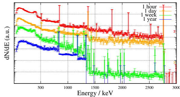
Figure 5: Photon spectra at a location close to the LBE dump at different decay times between 1 hour and 1 year.
