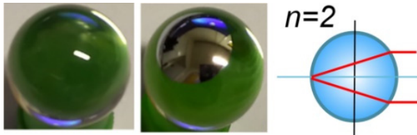
Figure 2: Glass ball reflector (uncoated, coated, principle).
