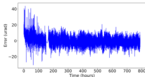
Figure 8: Error between the FSI inclinometer and Sherborne LSOC-1 inclinometer.
