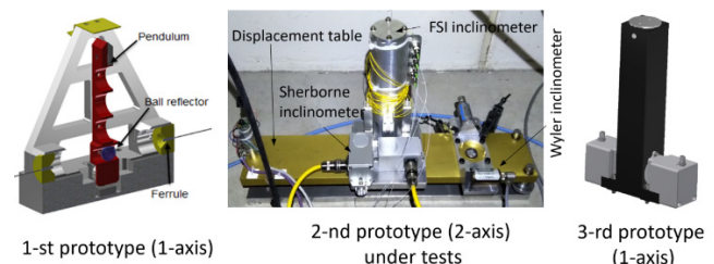
Figure 6: Family of FSI inclinometers developed and tested at CERN.
