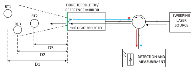
Figure 1: Multi-target Frequency Sweeping Interferometer schematic.
