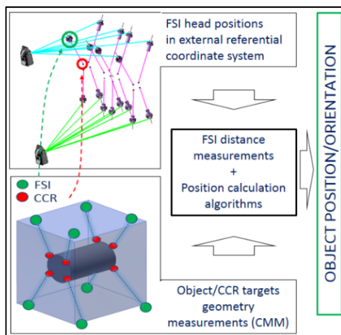
Figure 3: Sequence of measurements for intra-cryostat position monitoring.
