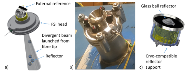
Figure 4: Intra-cryostat position monitoring instrumentation: a), b) FSI divergent beam head; c) cryo-compatible FSI reflector.
