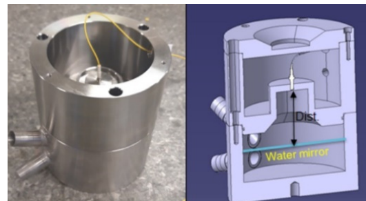
Figure 5: FSI-HLS sensor and its operation principle.
