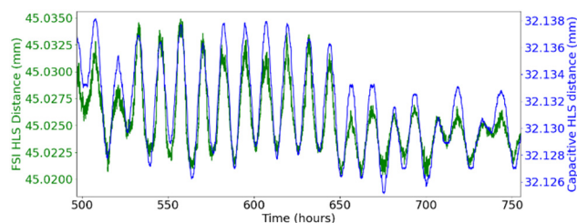
Figure 7: Comparison between an FSI-HLS sensor and a commercial capacitive HLS sensor.
