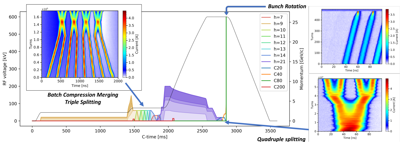
Figure 1: The momentum (black) and RF program (colored) for the BCMS cycle. The RF harmonics h = 7 to 21 (10 MHz) are handled by tunable ferrite loaded cavities while the other harmonics h = 42 (20 MHz), h = 84 (40 MHz) and h = 168 (80 MHz) are generated by fixed frequency RF systems. For each manipulation the evolution of the bunch profiles is shown.
