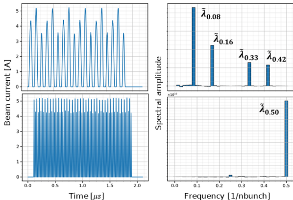
Figure 2: Effect of RF phase errors during the triple (top, h = 7 \rightarrow 21 ) and last (bottom, h = 42 \rightarrow 84 ) double splittings. The beam current (left) is analyzed with DFT (right) to identify the phase errors.
