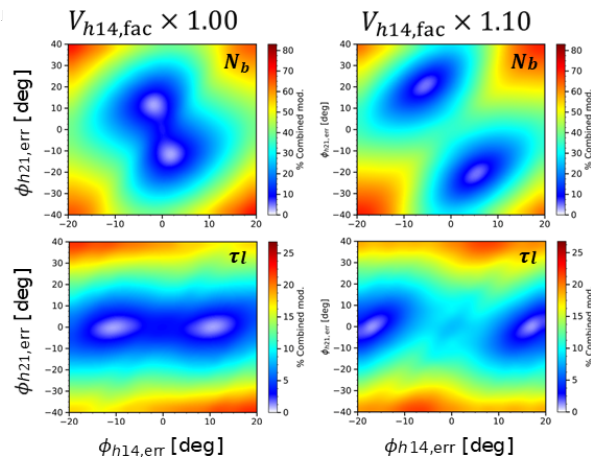
Figure 4: Map of the objective function minimizing \sum \tilde{\lambda}^2 for the triple splitting, without beam loading. The target spread to reduce is intensity (top) or length (bottom), for the nominal voltage at h = 14 (left) or increased by 10% (right).
