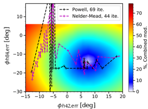
Figure 3: Scan of parameters to obtain the f objective function to minimize bunch intensity spread during the double splittings (colors) with the path of the optimization algorithms (black, purple), including beam loading.
