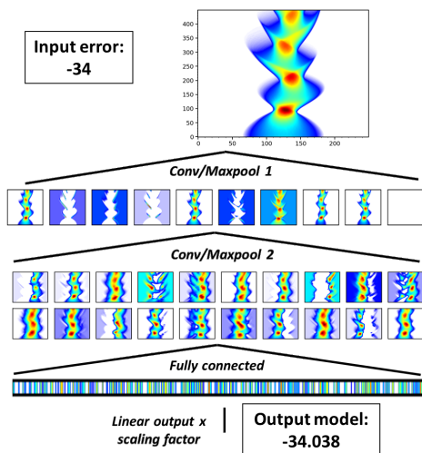
Figure 5: Convolutional Neural Network trained to identify relative phase errors between 40 MHz and 80 MHz voltages during bunch rotation from bunch profiles.
