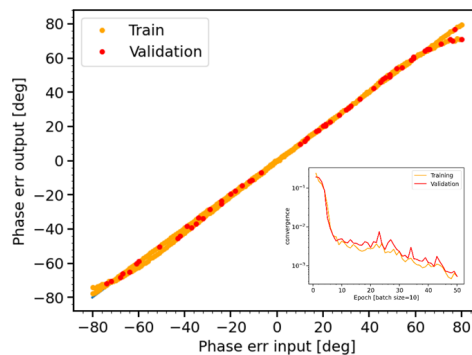
Figure 6: The phase of the 80 MHz voltage as obtained from the CNN compared to the expected phase error. The convergence (inlay plot) is displayed for both training and validation data with no sign of overfitting.
