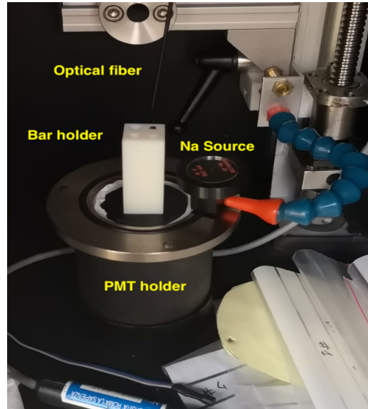
Figure 9: Experimental setup used to measure the single crystal bar LO and \tau , showing a crystal bar placed in the plastic holder over the PMT window. The optical fiber coupled to a blue LED and the support for the ^{22}\text{Na} source are visible too.
