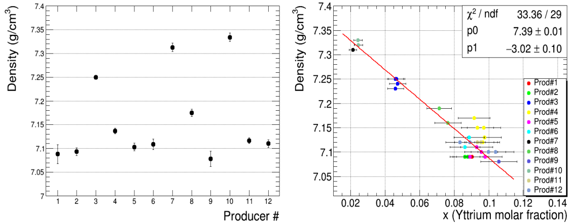
Figure 4: The mean density of the 15 bars is shown for each producer. The relative standard deviation of the bar density is well below 1 % for all producers (left). Crystal density as a function of the Yttrium molar fraction ( x ) for a subsample of the crystal bars analyzed in this study. The linear correlation is clearly visible (right).
