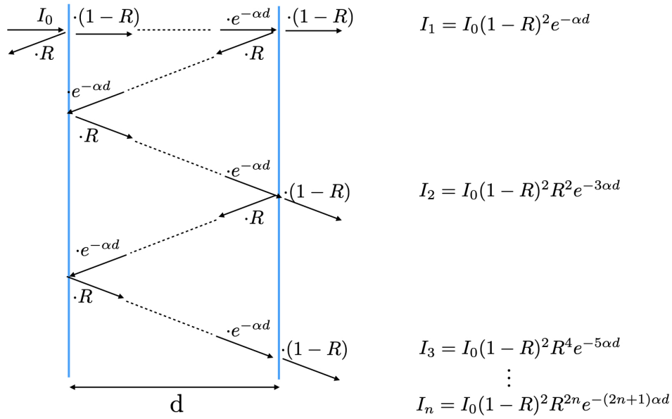
Figure 22: Sketch of the multiple reflection of the light between parallel crystal faces at a distance d . The analytical expressions for the contributions of the reflected, absorbed and transmitted light are also reported along the light path.
