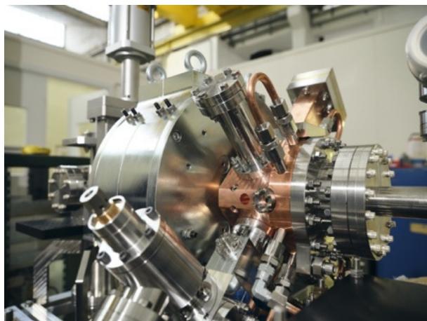
Figure 3: Electron source prototype for Run 2c.
