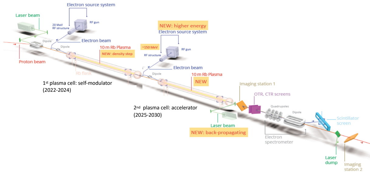
Figure 2: Schematic of the AWAKE Run 2c and 2d layout.
