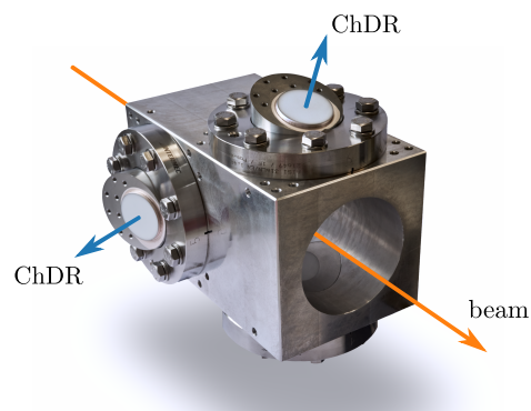
Figure 6: Schematic of ChDR pick-up using alumina rods.
