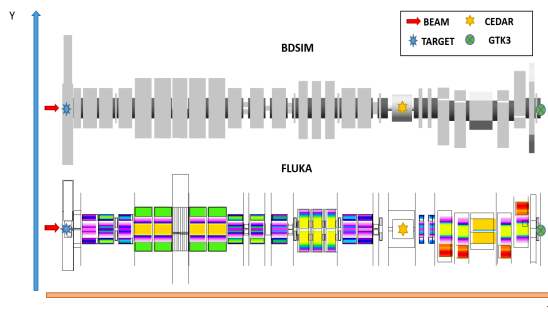
Figure 3: K12 model in BDSIM and FLUKA. In FLUKA the magnets fields are shown as well.
