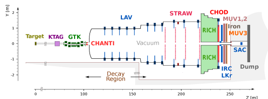
Figure 1: Scheme of the K12 beamline and the NA62 detector [1].
