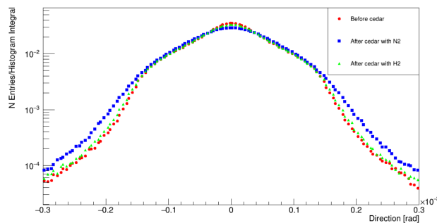
Figure 6: Angular spread of the beam before CEDAR and after CEDAR with N_2 and H_2 . Simulations in BDSIM.
