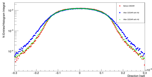
Figure 5: Angular spread of the beam before CEDAR and after CEDAR with N_2 and H_2 . Simulations in FLUKA.
