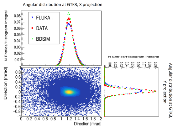
Figure 4: Angular distribution of the beam at the GTK3. 2D histogram for data, projections in X and Y for data, BDSIM and FLUKA.
