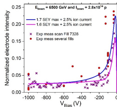
Figure 4: Variation of I_+/I_{electrons} vs V_{bias} : experimental data (red circle recorded during different fills and purple cross for a voltage bias scanning during the fill 7328) and calculated values for several SEY (color lines) considering an ion current of 2.5% of the total electron one.
