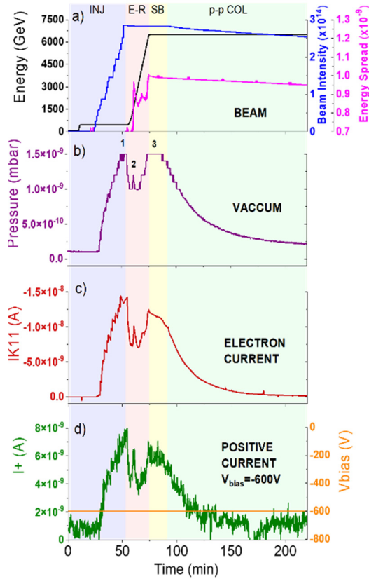
Figure 1: Measurements performed in station 4 of VPS during the Fill 7319: “blue” beam parameters (a), pressure (b), electron current (c) and positive current (d).
