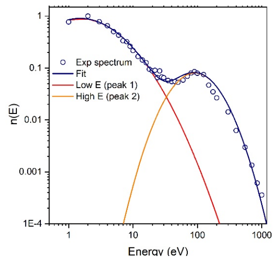
Figure 2: Normalized energy spectrum of electrons n(E) (blue open circle) recorded by an electrode in station 4 during a fill at 6500 GeV [4]. Lines are fits to experimental data with Eq. (3): total spectrum (blue line), low energy part (red line) and high energy part (yellow line).
