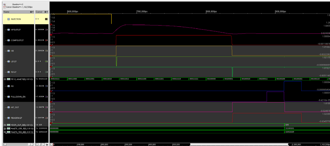
Fig. 4. Mixed-mode simulation using the post-layout view of a pixel: INJECTION is the test pulse from the calibration circuit; HPOUT the shaped signal at the comparator input; COMPOUT the comparator output; LE and TE the leading and trailing edges sensed by the digital readout electronics; TS the time-stamp; RD and PULLDOWN_EN digital signals sent to the pixel to store the pixel address and time-stamps in the corresponding EOC; HIT_OUT the output of the priority circuit connected to the following pixel in the double column; and READEN the output of the priority circuit connected to the digital readout of the pixel. The last three waveforms (figure bottom) correspond to the pixel address, and leading and trailing edge time-stamps.
