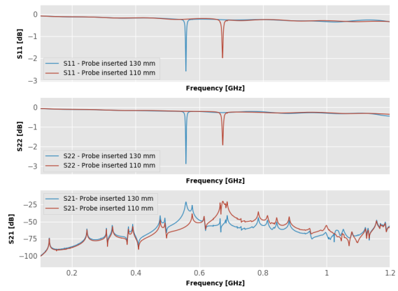
Figure 3: Simulated reflection parameters (S11, S22) and transmission parameters (S21) versus frequency for two different probe positions in the TCSPM. Probe-related modes are visible in reflection, while collimator-related modes are mainly observed in transmission.
