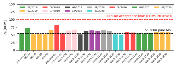
Figure 1: Electrical resistivity of Mo coated samples measured following the TCSPM production.
