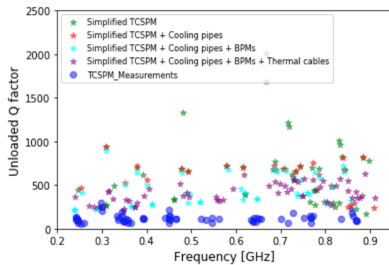
Figure 7: Simulated Q factors for different complexity of the TCSPM compared to measurements at 10 mm half-gap.
