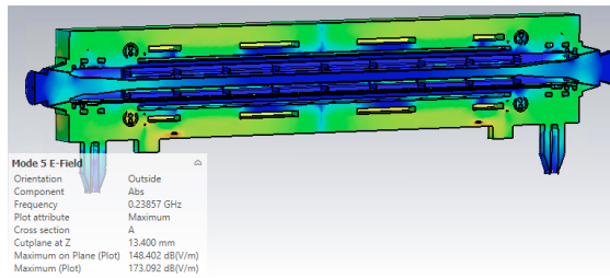
Figure 6: Electric field distribution of the mode at 239 MHz for 10 mm half-gap position.
