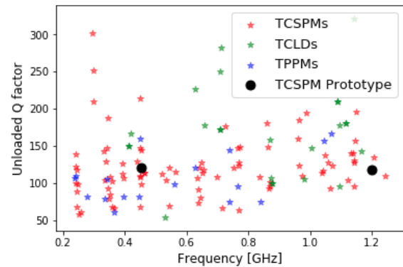
Figure 4: Measured Q factors versus frequency of TCSPM, TCLD, TCPPM and TCSPM prototype collimators for 10 mm half-gap.
