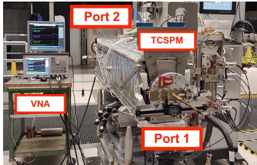
Figure 2: The TCSPM collimator together with the RF measurement setup. Ports 1 and 2 are the VNA ports used for probe reflection and transmission measurements.
