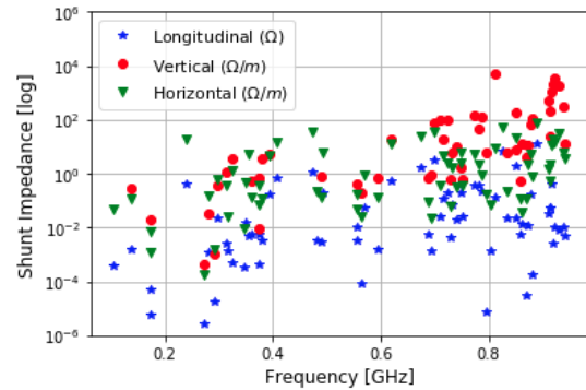
Figure 8: Simulated longitudinal and transverse TCSPM shunt impedances, for 10 mm half-gap.
