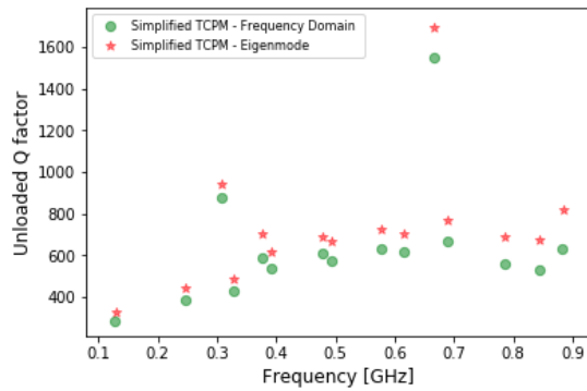
Figure 5: Unloaded Q factors simulated with Eigenmode and FD solvers for 10 mm jaw half-gap position of the TCSPM.
