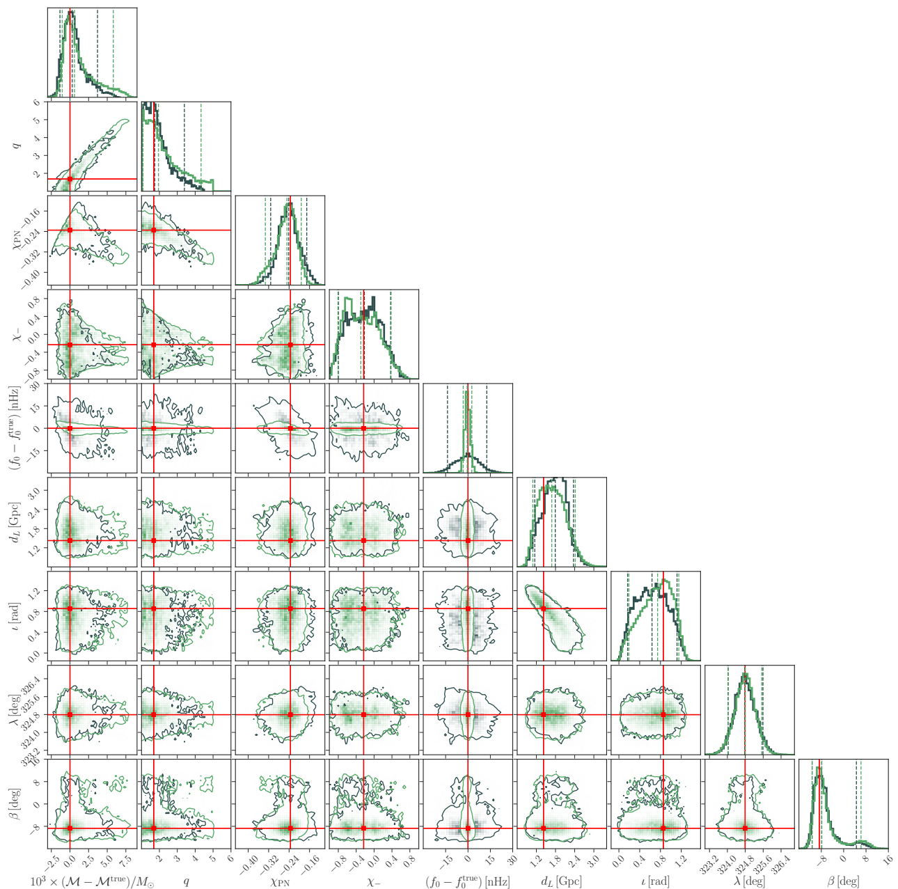
FIG. 6. Overplotting the uncertainties contours in the parameters of the GW190521-like binary (excluding AGN-related parameters) in the presence of the SMBH (green) and in its absence (in black). Red crosses denote the position of the true (cosmologically redshifted) parameters, while the dashed vertical lines indicate 90% CLs..
