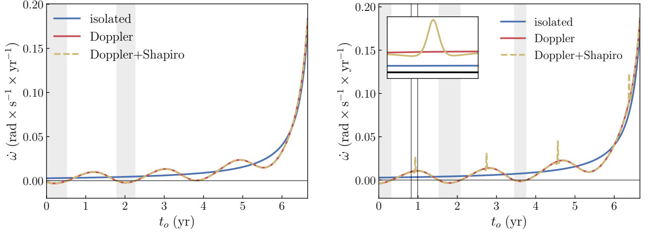
FIG. 4. The second derivative of the GW phase \ddot{\omega} \equiv \frac{d}{dt}\dot{\omega} = \frac{d^2}{dt^2}\varphi(t+d_{\text{effect}}(t)) in isolation and in the presence of the Doppler and Shapiro effects. We compare a system with large ( \iota_* = \pi/6 rad = 30 deg, left) and small ( \iota_* = -0.05 rad \approx -3 deg, right) outer orbit inclination. The remaining system parameters and plot features are the same as in Fig. 3. The figure on the right includes a zoom-in of the region marked by vertical lines, corresponding to a month around the moment the source is aligned behind the SMBH. At each passage, the Shapiro effect is strongly enhanced in the small inclination case. Note that at small inclinations the effect of lensing, not included here, would also be significant.
