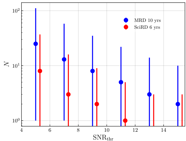
FIG. 1. Left: distribution of the SNR in LISA for GW190521, averaged over the sky position and polarization assuming that the binary merges shortly after 10 years of LISA observations. Solid lines correspond to SciRD detector sensitivity, while dashed lines corresponds to the current-best-estimate (CBE) sensitivity, similar to MRD at high frequencies. Right: number of GW190521-like events detectable by LISA as a function of the SNR threshold, for a fiducial (SciRD, 6 yrs) and optimistic (MRD, 10 yrs) mission configuration. SciRD points are shifted for clarity. Both panels assume a conservative duty cycle of 75%.
