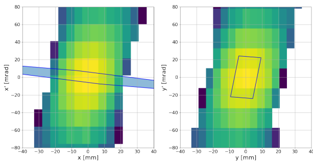
Figure 2: The produced particles' phase-space overlaid with the accepted phase space of the beamline. On the left is the horizontal plane and on the right that of the vertical plane.
