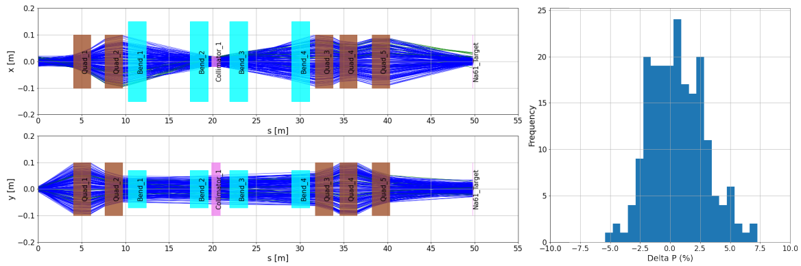
Figure 1: Tentative optics for the new low energy branch of the H2 line in EHN1. The horizontal plane is shown in the top plot on the left and the vertical plane shown lower left plot. The secondary target ends at s = 0 . The blue lines represent particle tracks and have been obtained using MAD-X's PTC code [10]. On the right is the momentum distribution of the particles which reach the end of the beamline with a 2 cm collimator opening.
