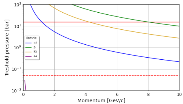
Figure 3: The threshold Cherenkov counter threshold curves for various particles. The solid red line is the maximum pressure of 15 bar, while the dashed red line represents the minimum pressure. Particles can be detected if threshold curve is below the maximum pressure.
