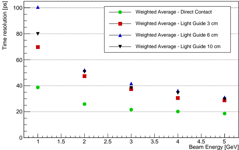
Figure 7: Time resolution of C&A GFAG combining the front and the back cells in direct dry contact with the MCD PMTs or using PMMA light guides. Employing a light guide worsens time resolution, but the deterioration depends little on the length.
