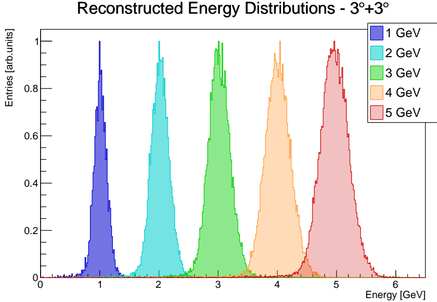
Figure 3: Distributions of the reconstructed energy at 3^\circ+3^\circ incidence angle rescaled to the same height.
