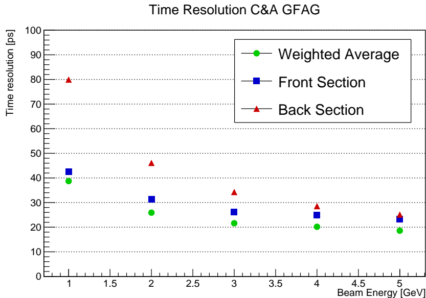
Figure 6: Time resolution of the GFAG cells with Hamamatsu MCD R7600U-20 PMTs in direct dry contact. The three set of resolutions are obtained using the front cell, the back one, and the inverse-variance weighted average of the two timestamps.
