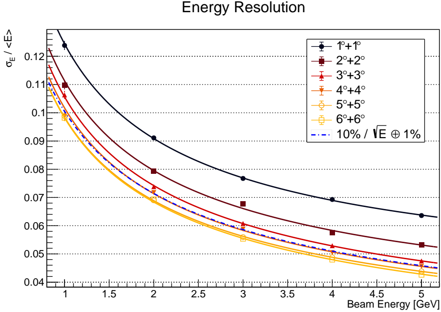
Figure 4: Energy resolution of the prototype measured at different incidence angles of the electron beam. The lines are fits of Eq. 3 to the datapoints. The common noise term is (0.024 \pm 0.004) GeV. The resolution improves with increasing incidence angle. This effect fades above 3^\circ+3^\circ . The blue dotted line is the resolution reached with 10% sampling and 1% constant terms.
