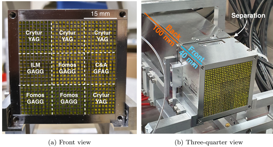
Figure 1: Pictures of the Tungsten-Crystal SPACAL prototype without readout. On the left, the 9 cells with different garnets and producers are highlighted. On the right, the front and the back sections are visible, with the small gap between the two and the mechanics holding the prototype.
