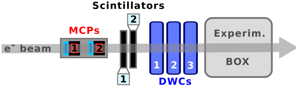
Figure 2: Test beam setup. The electron beam moves from left to right, two MCPs provide the time reference, two scintillating pads the trigger signal, and three DWCs the tracking information. The experimental box contains the prototype and the rotating steppers.
