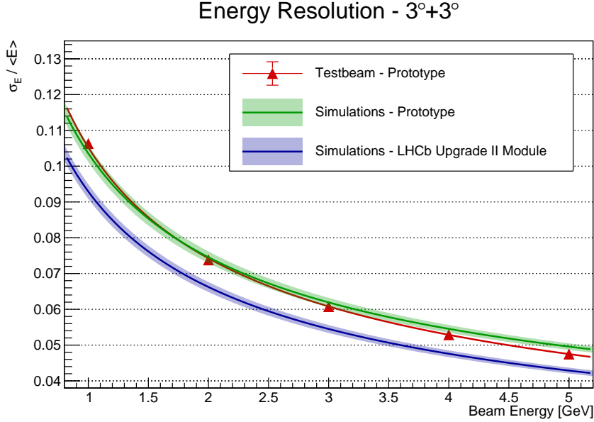
Figure 5: Energy resolution to electrons at 3^\circ+3^\circ incidence angle. Comparison between testbeam measurements of the prototype, simulations of the prototype, and simulations of the module designed for the LHCb Upgrade II [4]. Simulations are drawn with a 2 standard deviations error band.
