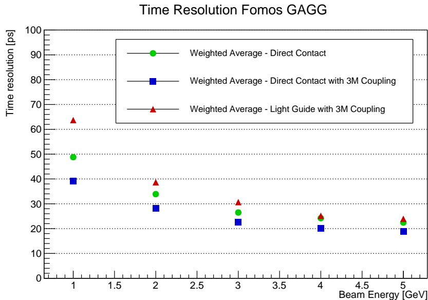
Figure 8: Time resolution of Fomos GAGG combining the front and the back cells coupled to the PMTs using a 3M optical adhesive with an index of refraction of 1.47.
