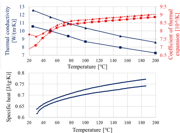
Figure 3: Min. and max. of measured thermomechanical material properties of isostatically pressed CMD10 ferrite: thermal expansion is measured for heating of samples.
