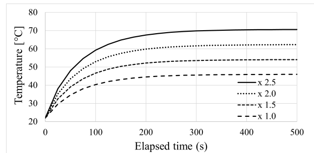
Figure 6: Predicted peak temperatures in the MKI Cool RF damper for different input powers.
