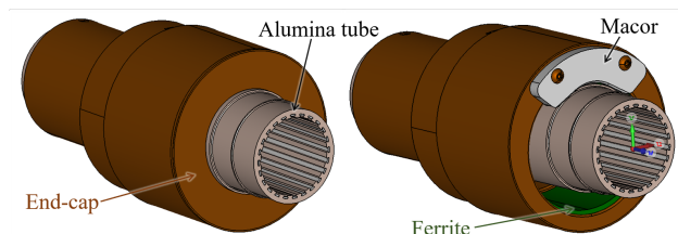
Figure 2: RF damper before (left) and after (right) modifications.
