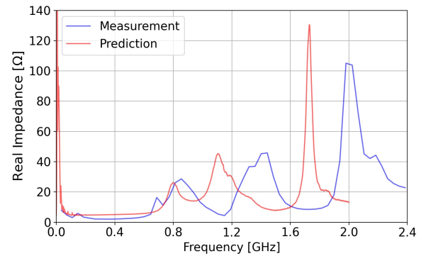
Figure 5: Predicted and measured real longitudinal beam coupling impedance of the MKI Cool.
