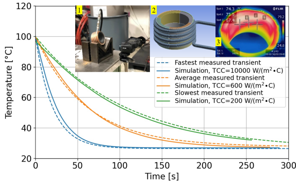
Figure 4: Measured cooling transients and corresponding simulations of the damper: TCC is tuned to agree with the measurement. (1) Measurement setup, (2) ANSYS simulation model, and (3) A thermal camera measurement.
