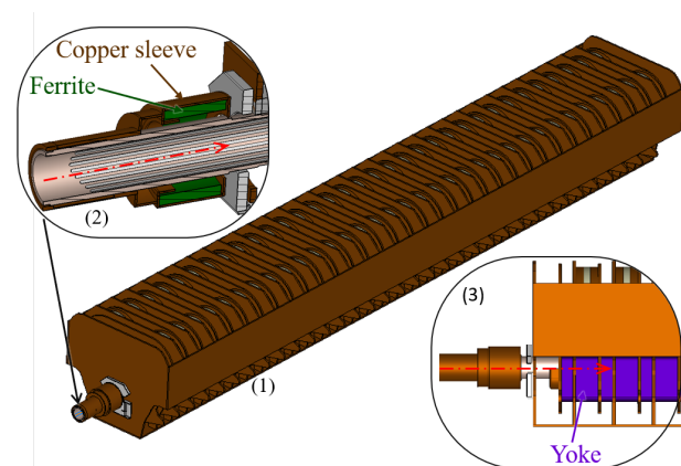
Figure 1: (1) The kicker magnet in its entirety, with the damper located on the left hand side. (2) Cross section of the damper (cooling pipes not shown). The red arrow indicates the direction of the beam. (3) External side view of the damper.
