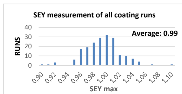
Figure 6: Histogram of maximum SEY for all coating runs.
