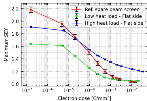
Figure 3: Conditioning curves of the high and low heat load beam screens. The conditioning curve of a reference beam screen (spare from the stock) is also shown for comparison.
