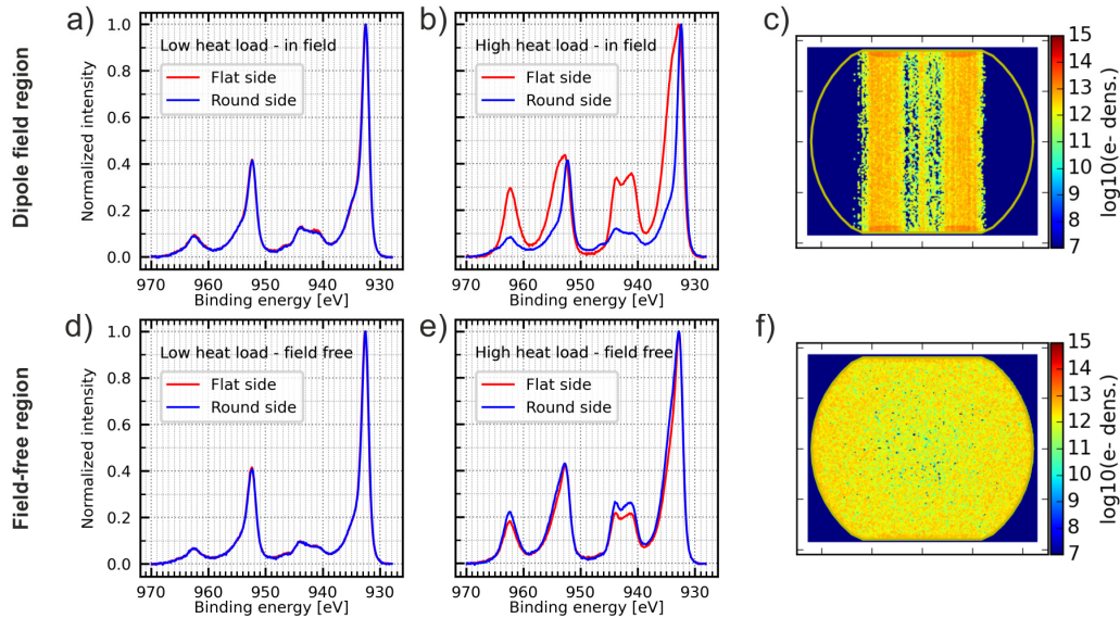
Figure 1: Cu 2p XPS spectra acquired on the low (a, d) and high (b, e) heat load beam screens, in different field configurations. The corresponding electron cloud density distributions from electron cloud build-up simulations [11] are shown for comparison (c, f).
