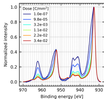
Figure 4: Cu 2p XPS spectra of the high heat load beam screen at different electron doses during conditioning.
