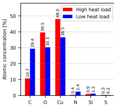
Figure 2: Elemental surface concentrations determined by XPS of the different beam screens surfaces (flat sides, in field region).
