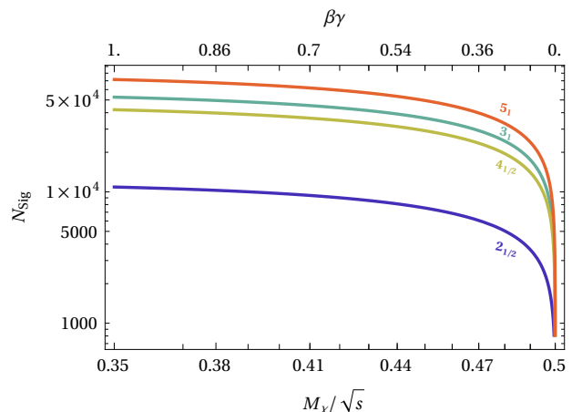
FIG. 5. Signal yield of the charged tracks for the 2_{1/2} , 3_1 , 4_{1/2} , 5_1 . The plot holds for all \sqrt{s} in the tens of TeV range, assuming the luminosity scales as Eq. 20. The cuts applied on the produced charged \chi 's are p_T > 200 GeV, |\eta_\chi| < 2 .
