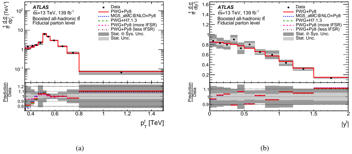
Figure 44: The normalized parton-level differential cross-sections are shown for (a) the transverse momentum of the randomly chosen top quark and (b) the absolute value of the rapidity of the randomly chosen top quark. The grey bands indicate the total uncertainty of the data in each bin. Data points are placed at the centre of each bin. The POWHEG+PYTHIA 8 MC sample is used as the nominal prediction to correct the data to parton level.
