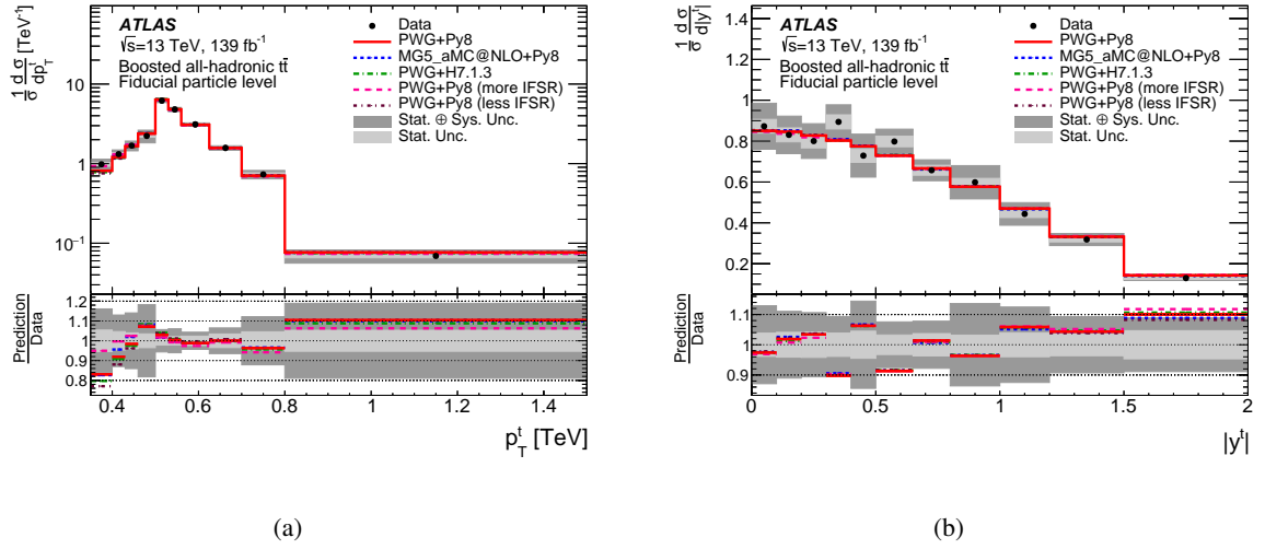
Figure 37: The normalized particle-level differential cross-sections are shown for (a) the transverse momentum and (b) the absolute value of the rapidity of the randomly chosen top-quark jet. The grey bands indicate the total uncertainty of the data in each bin. Data points are placed at the centre of each bin. The POWHEG+PYTHIA 8 MC sample is used as the nominal prediction to correct data to particle level.
