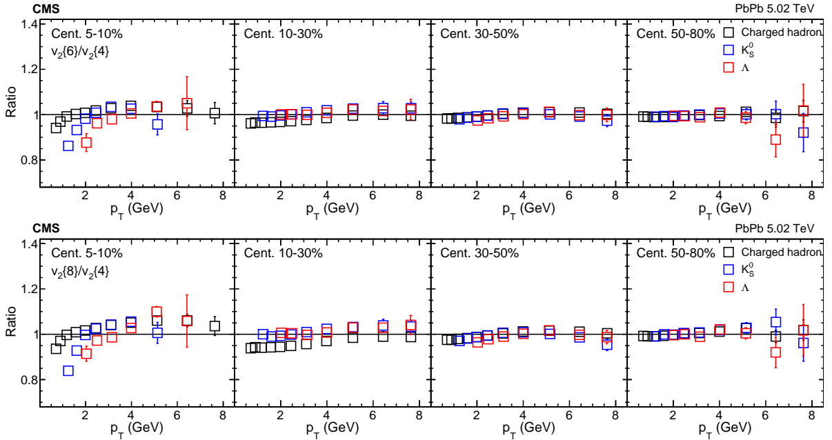
Figure 10: The v_2\{6\}/v_2\{4\} (upper) and v_2\{8\}/v_2\{4\} (lower) ratios in PbPb collisions at \sqrt{s_{\text{NN}}} = 5.02 TeV for charged hadrons, K_S^0 mesons, and \Lambda baryons in different centrality intervals. The vertical bars show the statistical uncertainties. The uncertainties are treated as uncorrelated for the ratios.
