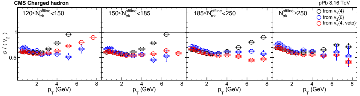
Figure 9: The v_2 fluctuation results of pPb collisions at \sqrt{s_{\text{NN}}} = 8.16 TeV for charged hadrons derived from different multiparticle correlations in different N_{\text{trk}}^{\text{offline}} ranges. The vertical bars and shaded boxes show the statistical and systematic uncertainties.
