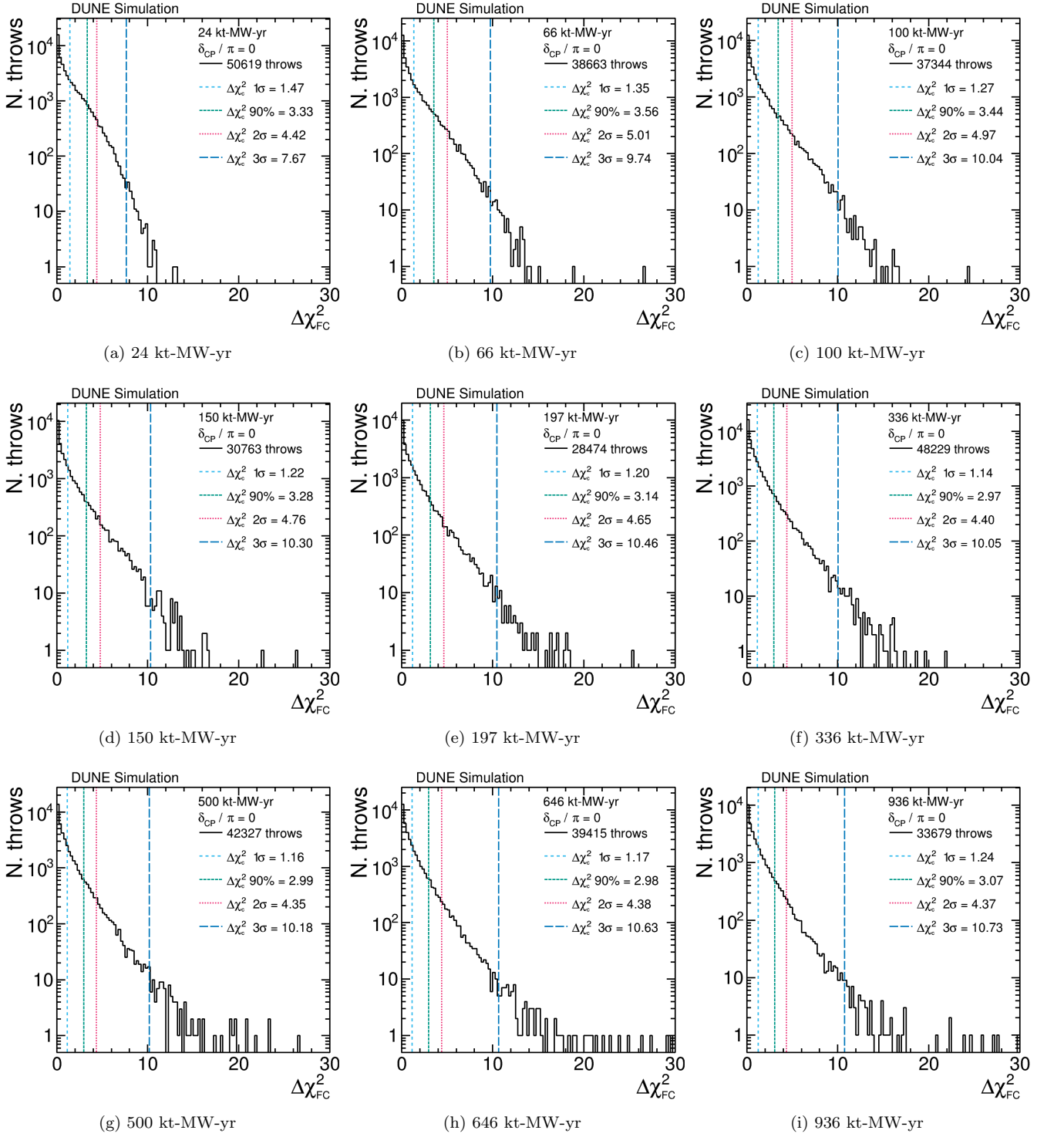
FIG. 19. Distribution of \Delta\chi^2 values, calculated using Equation 5, for a large number of throws with true \delta_{CP} = 0 , for a variety of exposures. The \Delta\chi^2_{FC} values (vertical lines) obtained using the Feldman-Cousins method show the \Delta\chi^2_{FC} value below which 68.27% ( 1\sigma ), 90%, 95.45% ( 2\sigma ) and 99.73% ( 3\sigma ) of throws reside, with the calculated values given in the legend. The number of throws used is also given.
