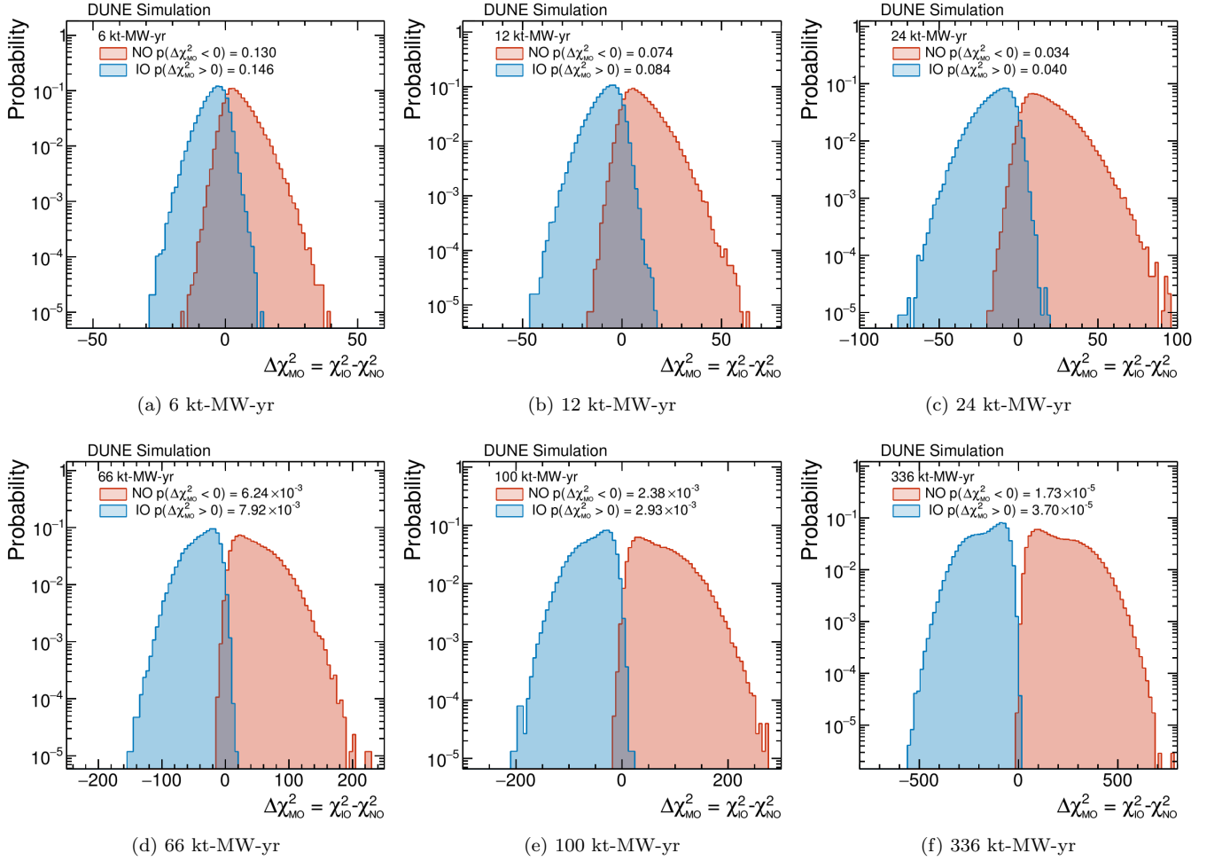
FIG. 16. The distribution of \Delta\chi_{\text{MO}}^2 = \chi_{\text{IO}}^2 - \chi_{\text{NO}}^2 values shown for both true normal (red) and true inverted (blue) hierarchies built using random throws of the systematic parameters, the oscillation parameters and with statistical variations. In each case, the \chi^2 values are separately minimized with respect to all variable parameters before calculating the test statistic. The fraction of throws for which the value of \Delta\chi_{\text{MO}}^2 is greater than (less than) 0 is also given for inverted (normal) hierarchies. For each ordering and exposure, approximately 100,000 throws were used.
