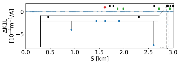
Figure 4: Quadrupole strengths required to reconstructed measured phase advance, including a zoom to the 2 powered correctors. The black and green bars show the location of horizontal and vertical collimators; the red marker the IK.
