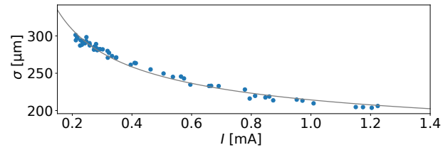
Figure 2: RMS BPM resolution ( \sigma ) over bunch current, using the first 1000 turns for analysis. The gray line is a fit of a function AI^{-1/2} + B .
