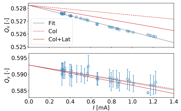
Figure 3: Horizontal (top) and vertical (bottom) tune over bunch current, for the fit, the expected collimator contribution (Col) and additional lattice contributions (Col+Lat).
