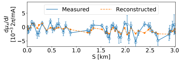
Figure 5: Measured and reconstructed horizontal phase advance over bunch current. BPMs with errors bars greater than \pm 1 \times 10^{-2} 2\pi/\text{mA} are not shown.
