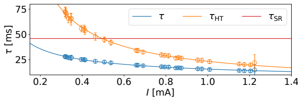
Figure 1: Measured damping time \tau , synchrotron radiation damping time \tau_{SR} and decoherence damping time \tau_{HT} over bunch current. The blue line is a fit of a function AI^{-1/2} + B ( A = 16.2 \pm 0.2 , B = -0.5 \pm 0.2 ) and the orange one of a function AI^{-1} + B ( A = 22.2 \pm 0.2 , B = 1.3 \pm 0.4 ).
