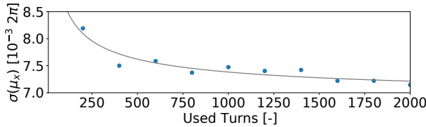
Figure 1: Horizontal rms phase advance error, \sigma(\mu_x) , for LER IK measurements for an optics with \beta_{x,y}^* = 80, 2 mm. The gray line is a fit of a function A \text{ turns}^{-1/2} + B .
