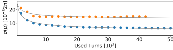
Figure 5: \sigma(\mu_x) (blue), \sigma(\mu_y) (orange) for measurements with PLL excitation in LER for an optics with \beta_{x,y}^* = 80, 1 mm. The gray line is a fit of a function A \text{ turns}^{-1/2} + B .
