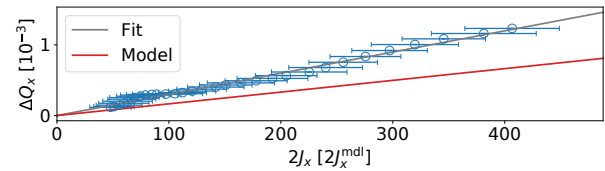
Figure 3: Horizontal amplitude detuning for LER optics \beta_{x,y}^* = 80, 1 mm.
