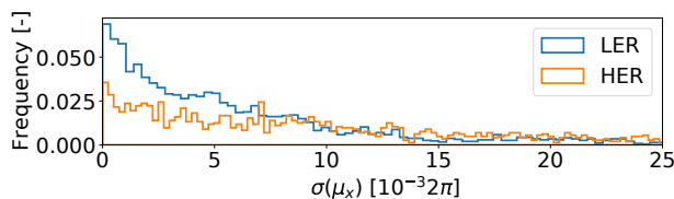
Figure 2: Horizontal rms phase advance error, \sigma(\mu_x) , for all BPMs using 2000 turns for IK measurements with \beta_{x,y}^* = 80, 2 mm.
