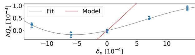
Figure 4: Chromaticity for HER with \beta_{x,y}^* = 80, 2 mm.
