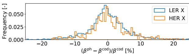
Figure 6: \beta -beating between COD and IK TbT measurements for LER (blue) and HER (orange).
