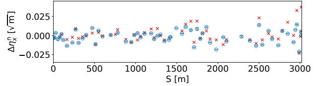
Figure 7: Horizontal \beta -beating (top) and \eta^n (bottom) with respect to the model for COD (red crosses) and TbT (blue circles) measurements for HER optics with \beta_{x,y}^* = 80, 2 mm.
