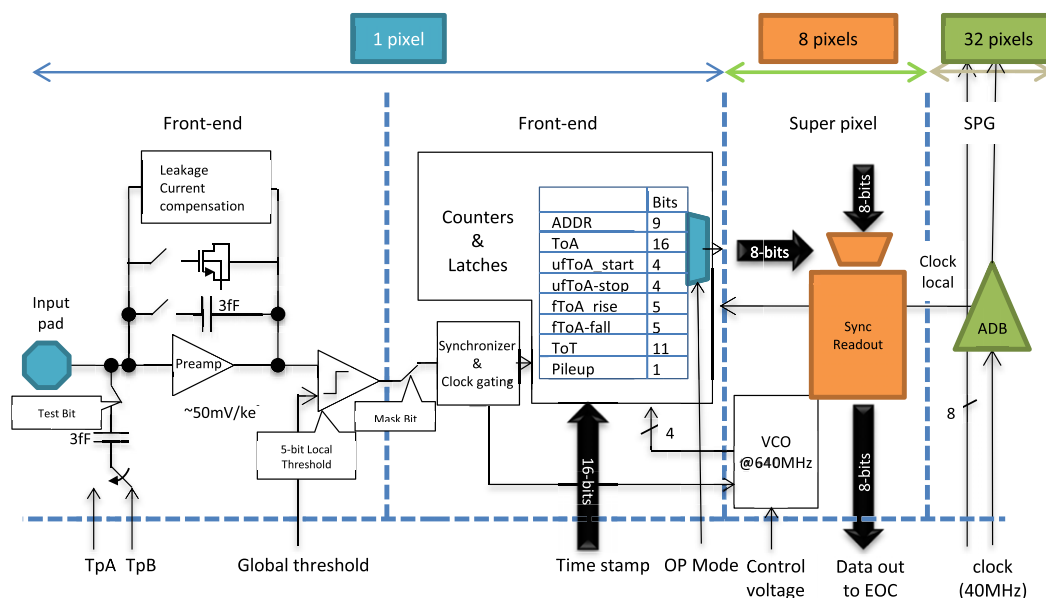
Figure 1. Schematic diagram of the Timepix4 front-end. The front-end of a single pixel is divided into an analog and a digital part. A superpixel consists of two by four pixels and contains a 640 MHz oscillator which is used for precise time measurements. A superpixel group (SPG) consists of four superpixels and contains two adjustable delay buffers (ADBs) that distribute the system clock along columns of pixels (only one is shown). Reproduced from [10]. © The Authors. Published by IOP Publishing Ltd on behalf of Sissa Medialab. CC BY 4.0.
