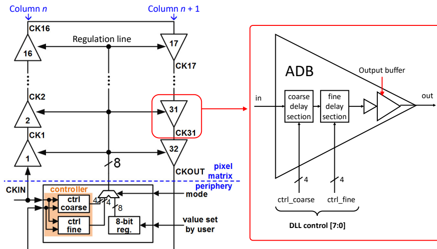
Figure 4. Schematic of the digital delay-locked loop that distributes the 40 MHz reference clock along a double-column. Reproduced from [18]. © 2019 IOP Publishing Ltd and Sissa Medialab.
