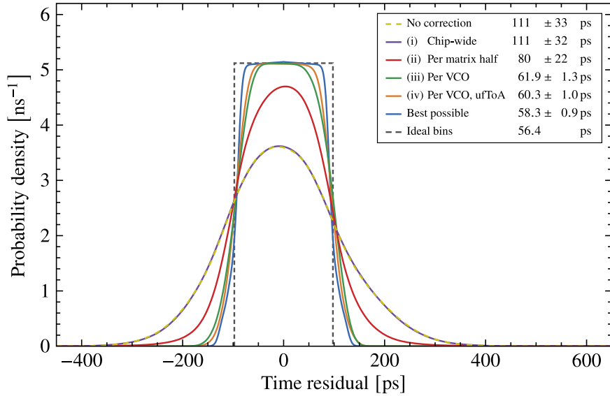
Figure 10. Expected time-residual distributions of the TDC based on the measured bin size structure of the Timepix4v2 device for various correction methods to compensate for VCO frequency variation and the ultra-fine bin structure. For each case the overall TDC resolution is presented in the legend, where the error indicates the RMS value over the pixels.
