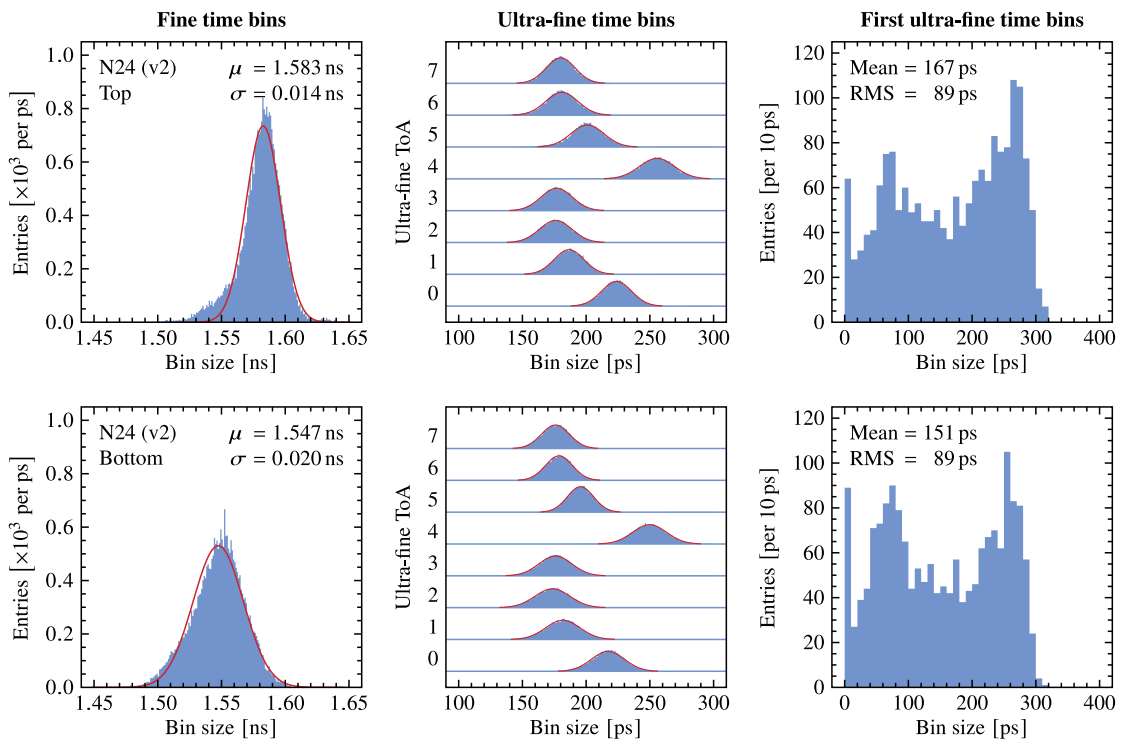
Figure 9. Distribution of fine time bin sizes the central fine time bins with 0 < \text{fToA} < 16 (left), the ultra-fine time bins (centre), and the first bins before a rising edge of the 40 MHz reference clock (right) for the top and bottom halves of a Timepix4v2 device.
