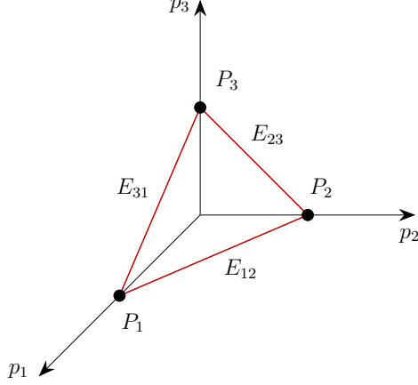
Figure 3: Sketch of the base \Delta of the torus fibration \pi : \partial X \rightarrow \Delta .
