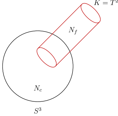
Figure 5: Sketch of the IIA setup of type 1) with “vector-like” flavor symmetry. The total geometry is T^*S^3 with N_c color D6-branes (black) wrapped on the compact S^3 and N_f flavor D6-branes (red) wrapped on T^2 \times \mathbb{R}_+ intersecting the S^3 in a circle and the boundary in T^2 .
