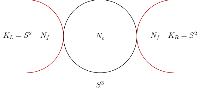
Figure 6: Sketch of the IIA setup of type 2) with chiral pairs. The total geometry is again T^*S^3 with N_c color D6-branes wrapped on the compact S^3 (black) and two stack of N_f flavor D6-branes (red) wrapped on two copies of \mathbb{R}^3 intersecting the S^3 in the north and south pole. These intersect the boundary in two two-spheres K_{L,R} .
