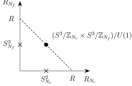
Figure 7: Sketch of an Acharya-Witten cone as a fibration over the quadrant R_{N_c}, R_{N_f} \geq 0 . The fibers are copies of (S^3/\mathbb{Z}_{N_c} \times S^3/\mathbb{Z}_{N_f})/U(1) . Whenever R_{N_c}, R_{N_f} = 0 fibers degenerate to two-spheres. The link of the cone at radius R projects to the dashed line.
