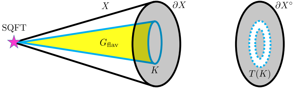
Figure 1: Depiction of an SQFT realized at a localized region of a non-compact geometry X , with boundary \partial X . Flavor branes can extend out to infinity and intersect the boundary along a subspace K . Our procedure for extracting the global form of the flavor symmetry, 1-form symmetry and possible 2-group structures involves working with \partial X^\circ = \partial X \setminus T(K) , where T(K) is a tubular neighborhood of K . The Mayer-Vietoris exact sequence then yields the relevant physical structures directly from geometry.
