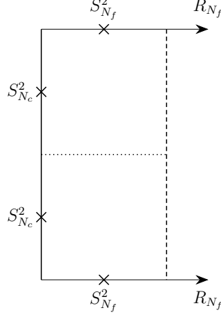
Figure 9: Gluing of two Acharya-Witten cones along a common subset of their boundary (dotted). The boundary of the new space is fibered over the dashed line.
