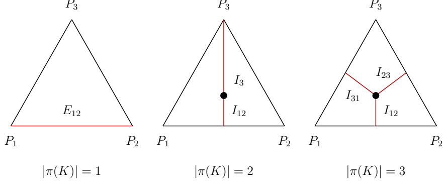
Figure 4: Sketches of the deformation retracts for the base \Delta . In the first and second and third configuration the orbifold locus projects to P_3 and P_1, P_2 and P_1, P_2, P_3 respectively. The T^3/\Gamma fibration then deformation retracts to a fibration over the graphs \mathfrak{G} marked red. We depict a decomposition of \mathfrak{G} into intervals I_* with one endpoint on the boundary of \Delta .
