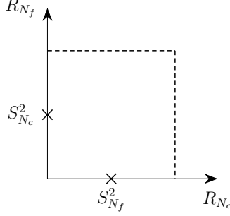
Figure 8: Alternative parametrization for the boundary of an Acharya-Witten cone.
