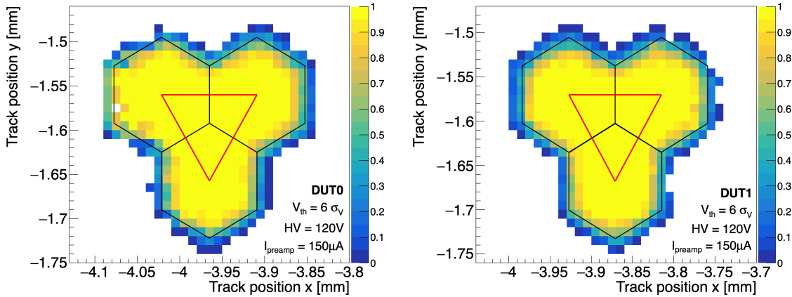
Figure 8. Efficiency map measured for DUT0 (left) and DUT1 (right) at I_{\text{preamp}} = 150 \mu\text{A} , threshold V_{\text{th}} = 6 \sigma_V and HV = 120 V. The pixel edges are shown by the black lines. The efficiency degradation around the external edges of the three pixels is due to the FEI4 telescope resolution. The efficiency measured inside the triangular area delimited by the red lines is unaffected by the telescope pointing resolution and is used throughout this study.
