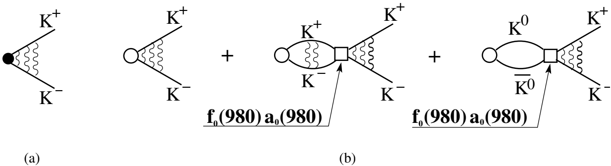
Fig. 2: The schematic description of K^+K^- production processes. a) The black point presents the pair point-like production; the wavy lines describe the Coulomb interaction in the final state. b) The circle and square present the pair non point-like production and strong interaction in the final state respectively.
