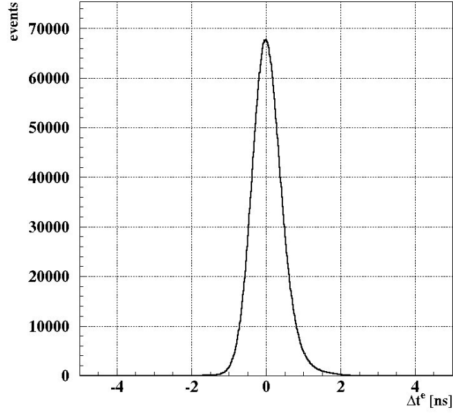
Fig. 4: \Delta t^e distribution of electron-positron pairs.
