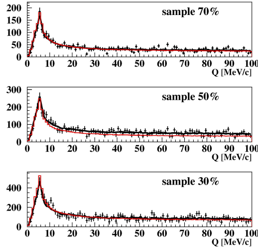
Fig. 7: Q distributions of the subsamples 30%, 50% and 70% for DATA1 and DATA2. Simulated distributions of K^+K^- (ALICE parametrization) and residual background of \pi^+\pi^- , accidental and p\bar{p} pairs are fitting the experimental spectrum in the interval 0 < Q < 100 \text{ MeV}/c . The red line is the K^+K^- distribution, the black line is the sum of K^+K^- and residual background. In the subsamples 70% and 30% the residual background is small and these lines practically coincide.
