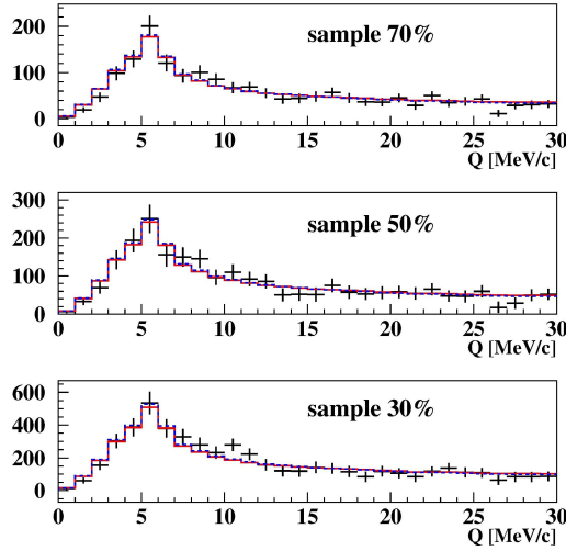
Fig. 9: Q distributions in the interval 0 - 30 \text{ MeV}/c of K^+K^- (ALICE parametrization) of the subsamples 30%, 50% and 70% for the DATA1 and DATA2 after residual background subtraction. The red and the blue fitting curves were evaluated from the analysis of experimental distributions with residual background in Coulomb and Martin parametrizations respectively. It is seen that in this interval of Q the difference between these curves is absent and they describe "pure" experimental K^+K^- distributions well.
