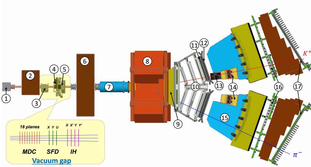
Fig. 1: General view of the DIRAC setup (1 – target station; 2 – first shielding; 3 – micro drift chambers (MDC); 4 – scintillating fiber detector (SFD); 5 – ionization hodoscope (IH); 6 – second shielding; 7 – vacuum tube; 8 – spectrometer magnet; 9 – vacuum chamber; 10 – drift chambers (DC); 11 – vertical hodoscope (VH); 12 – horizontal hodoscope (HH); 13 – aerogel Cherenkov (ChA); 14 – heavy gas Cherenkov (ChF); 15 – nitrogen Cherenkov (ChN); 16 – preshower (PSh); 17 – muon detector (Mu).
