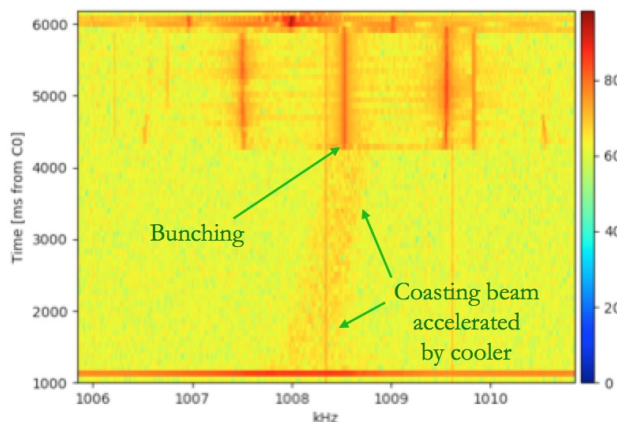
Figure 6: Longitudinal Schottky spectra of a coasting H^- beam under electron cooling.
