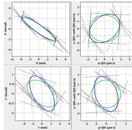
Figure 3: Transverse phase space reconstruction using the measured beam sizes from Fig. 2.
