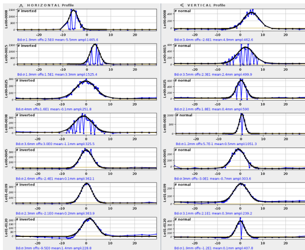
Figure 2: Profile measured with subsequent profile monitors along a straight transfer line from the extraction towards the old experimental area.
