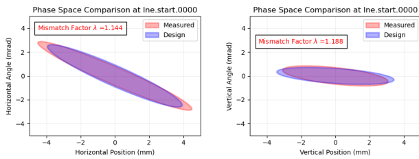
Figure 5: Comparison of phase space ellipses from the quadrupole scan shown in Fig. 4 with theoretical ones.
