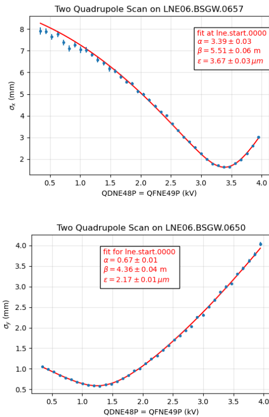
Figure 4: Typical quadrupole scans to characterise the beam done towards the end of the ASACUSA 1 line.
