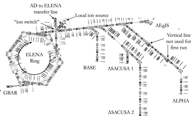
Figure 1: Layout of the ELENA ring and transfer lines.
