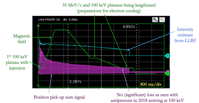
Figure 7: Cycle with H^- acceleration followed by deceleration to prepare antiproton operation.
